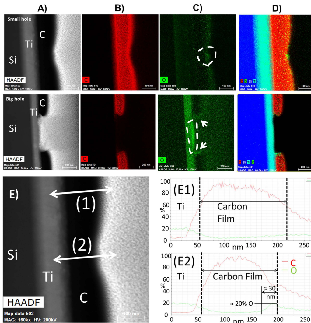
Figure 5. EDX chemical mappings on two craters to study the oxygen concentration. Top row: 3.9 \cdot 10^6 \text{ J} \cdot \text{mm}^{-2} . Bottom row: 3.4 \cdot 10^7 \text{ J} \cdot \text{mm}^{-2} . (A) STEM micrographs. (B) Carbon elemental map. (C) Oxygen elemental map. (D) Relative map showing the distribution of each element with the sample with carbon in red, silicon in dark blue, titanium in light blue and oxygen in green. (E) EDX-STEM line scan analysis on two different positions, far and close to the beam center, for the spot annealed with an energy density of 3.9 \cdot 10^6 \text{ J} \cdot \text{mm}^{-2} (E1) Carbon (in red) and oxygen (in green) concentrations recorded along the white arrow labeled (1). (E2) Carbon (in red) and oxygen (in green) concentrations recorded along the white arrow labeled (2).
