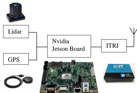
Figure 10: Perception Unit System Architecture.
