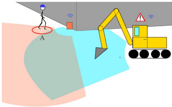
Figure 16: Shared perception between a perception unit and a digger. The field of perception of the unit is in orange, the one of the digger in blue. The worker is seen by the perception units that sends its location to the connected digger.
