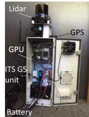
Figure 9: Perception unit hardware components.
