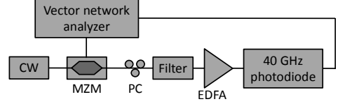
Fig. 2. Experimental set-up for characterization of the filter response.
