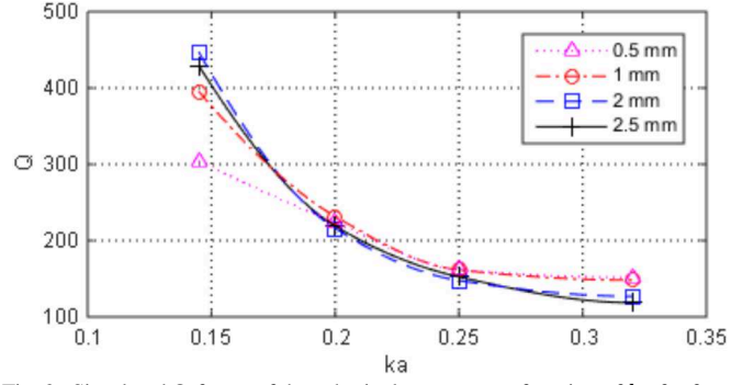
Fig. 9. Simulated Q-factor of the spherical antenna as a function of ka for four different diameters.
