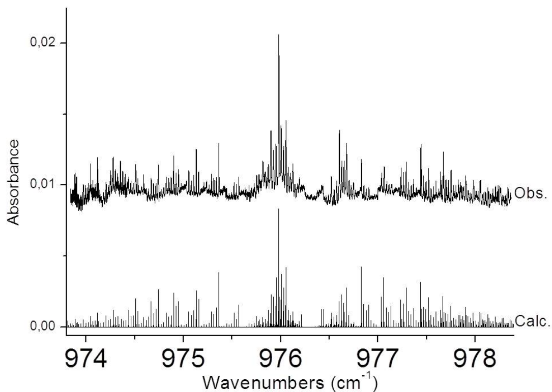
Figure 6: Comparison between the observed jet-cooled EC-QCL spectrum of the \nu_{\text{as}} band and a simulated stick spectrum of the \nu_{\text{as}} modes of both isotopologues without the contribution of the hyperfine structure (using set of parameters 1 and 3 of Table 2), at a rotational temperature of 6 K.
