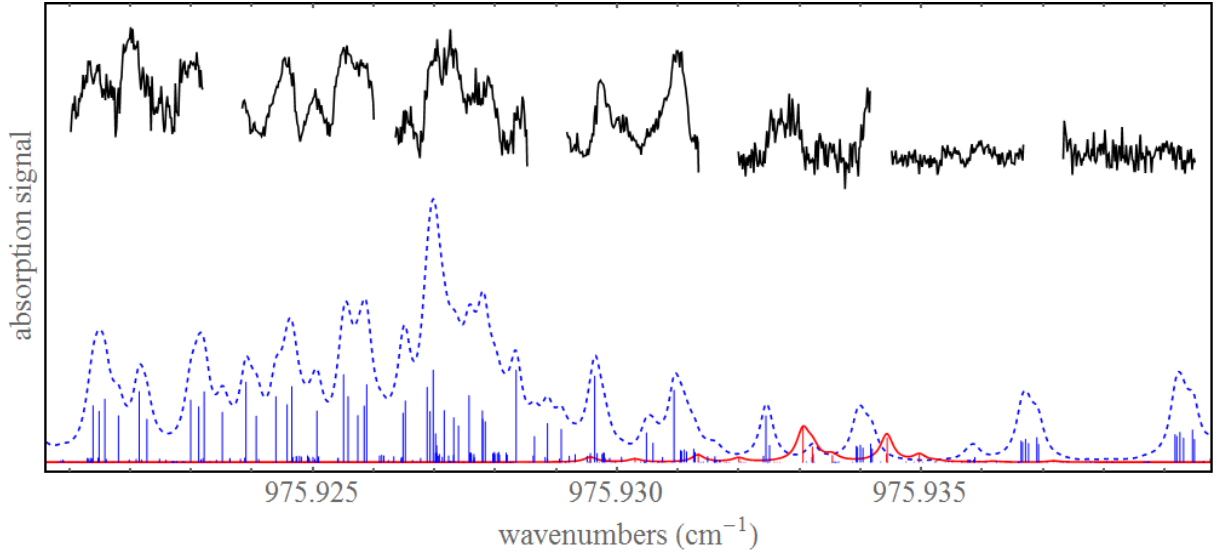
Figure 9: Upper black curve: linear absorption spectroscopy of an MTO-seeded continuous skimmed supersonic beam, in the vicinity of the R(20) \text{CO}_2 laser line frequency (located at \sim 975.93044 \text{ cm}^{-1} ); experimental conditions: 100 \mu\text{m} nozzle diameter, 750 \mu\text{m} skimmer diameter, helium backing pressure \sim 1 bar, oven temperature \sim 90^\circ\text{C} , translational longitudinal temperature \sim 1 K, 9 mm nozzle-to-skimmer distance, 1 point recorded every 100 kHz, \sim 1 s of integration time per point, 1.5 \times 10^{-5} \text{ cm}^{-1} binning, \sim 0.5 \mu\text{W} of laser power in each of the 18 passes on the multi-pass cell (see text), \sim 5 mm beam waist. Dashed blue curve: simulated \text{CH}_3^{187}\text{ReO}_3 spectrum at a rotational temperature of 15 K, using set of parameters 2 of Table 2. Solid red curve: simulated \text{CH}_3^{185}\text{ReO}_3 spectrum at a rotational temperature of 15 K, using set of parameters 4 of Table 2. Stick spectra (blue for \text{CH}_3^{187}\text{ReO}_3 and red for \text{CH}_3^{185}\text{ReO}_3 ) are convolved by a Lorentzian profile of full-width-at-half-maximum 2.5 \times 10^{-4} \text{ cm}^{-1} , corresponding to the expected Doppler broadening resulting from the divergence of the beam. 9
