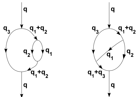
Figure 8: The two diagrams of order 4 in \hat{V} that may contribute to the damping rate \Gamma_{\mathbf{q}} of the phonon \mathbf{q} to the order q^7 thanks to the “small denominator” effect. The one on the left (I) is a Beliaev process with a single loop correction (itself of the Beliaev nature) to the virtual phonons angular eigenfrequency. The one on the right (II) is a Beliaev process enriched by an interaction between the virtual phonons. Each vertex corresponds to an action of \hat{H}_3^{(\pm)} .
