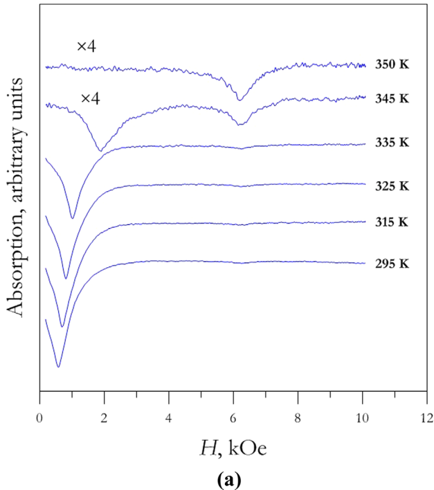
Fig. 9. EMR spectra series for the synthesized sample at \nu \approx 17 (a) and 24.5 GHz (b) and different temperatures shown alongside the curves.
