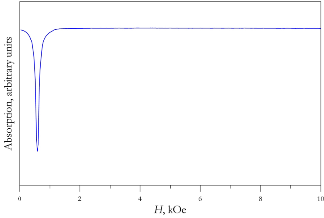
Fig. 8. EMR spectrum of \text{FeBO}_3 single crystal at 17GHz and 293 K. The magnetizing field is applied in the basal plane.
