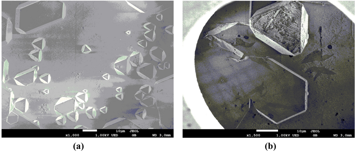
Fig. 5. Electron microscope pictures taken with a field emission SEM JSM-7800F microscope, showing FeBO 3 film on GaBO 3 substrate for two different magnifications.
