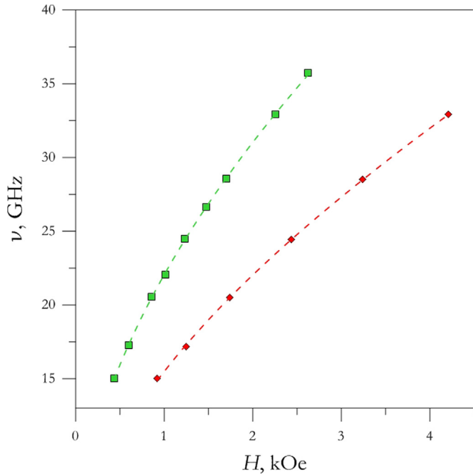
Fig. 10. Dependence of the AFMR frequency on the magnetizing field for FeBO 3 film at 300 (squares, green online) and 340 (diamonds, red online) K. The dashed curves are fittings according to Eq. (4). (For interpretation of the references to color in this figure legend, the reader is referred to the web version of this article.)
