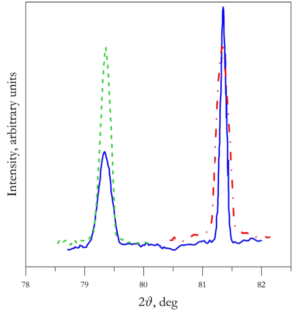
Fig. 7. XRD pattern of a synthesized sample (continuous, blue online) compared to those of FeBO 3 (dashed, green online) and GaBO 3 single crystals (dash-dotted, red online). (For interpretation of the references to color in this figure legend, the reader is referred to the web version of this article.)
