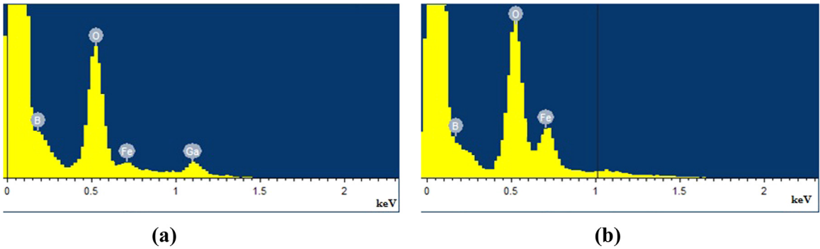
Fig. 6. EDS spectra of a typical sample. The electron beam is focused on the surface of the substrate (a) or on that of the film (b).
