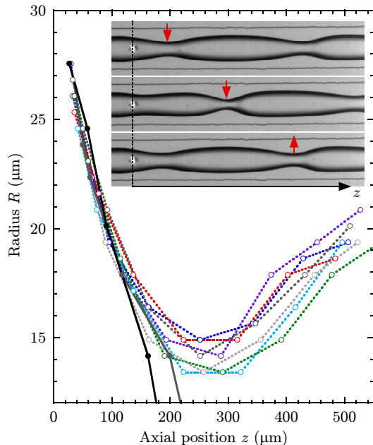
Figure 3. Evolution of the minimal thread radius R along the propagation axis z (origin at the laser spot) of seven distinct pinching events not leading to the fragmentation (open symbols, dotted lines), and the two first breakup events under the same experimental conditions (filled symbols, solid lines). The red, downwards and upwards vertical arrows highlight a specific neck pinching, successively amplifying and decaying. Laser power P = 24 mW, flow rates (Q_w, Q_o) = (2, 1) \mu\text{L min}^{-1} .
