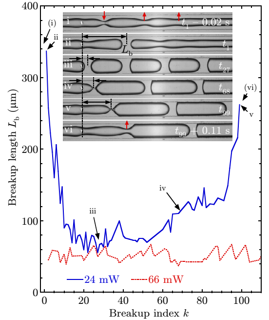
Figure 4. Evolution of the breakup length L_b in a succession of breakup events, for two distinct laser powers, in the transient fragmentation regime [24 mW, analogous to Fig. 2 (a), top], and in the stationary regime [66 mW, as in Fig. 2 (a), bottom]. Images i–vi refer to the transient case represented (24 mW), for several distinct breakup events k at the corresponding instants t_k . The red, downwards and upwards vertical arrows depict amplifying and decaying pinchings, respectively. In all cases, (Q_w, Q_o) = (2, 1) \mu\text{L min}^{-1} .
