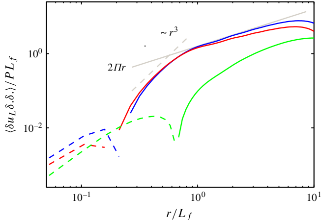
FIGURE 12. Plot of J_K (red), J_P (green) and J_K + J_P (blue) for run Q1-SS ( k_f = 54 ): —, positive values; - - - -, negative values. Solid grey line, (3.3); dashed grey line to aid the reader, \sim r^3 .
