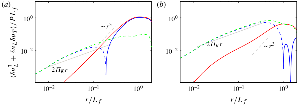
FIGURE 8. Decomposition of \langle \delta u_L \delta \mathbf{u} \cdot \delta \mathbf{u} \rangle (blue) into its geostrophic component (red) and ageostrophic component (green). (a) Q1 and (b) M1. Solid lines: positive values; dashed lines: negative values. Grey lines are shown to aid the reader: solid, 2\Pi_K r ; dashed, \sim r^3 .
