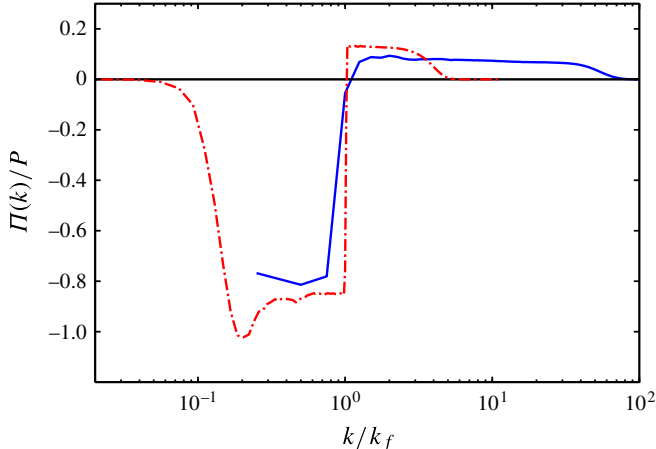
FIGURE 11. (Colour online) Total energy flux normalized with the total energy input P for Ro = 0.1 . —, Run Q1 ( k_f = 4 ); - - -, run Q1-SS ( k_f = 54 ).
