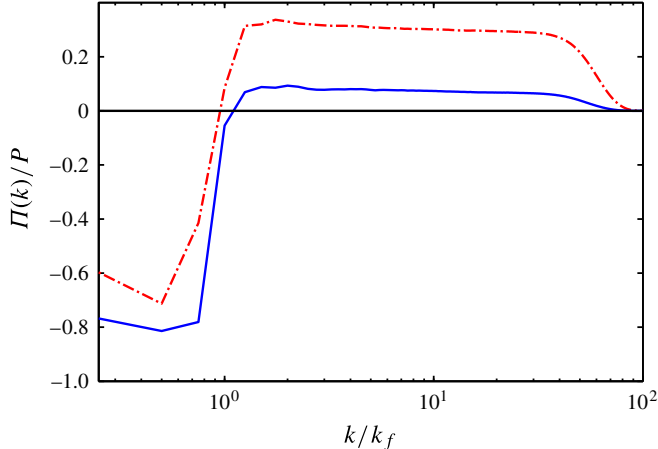
FIGURE 3. (Colour online) Total energy flux normalized with the total energy input P for —, Q1 ( Ro = 0.1 ) and -·-, Q2 ( Ro = 0.2 ). The forcing scale is at k_f = 4 .
