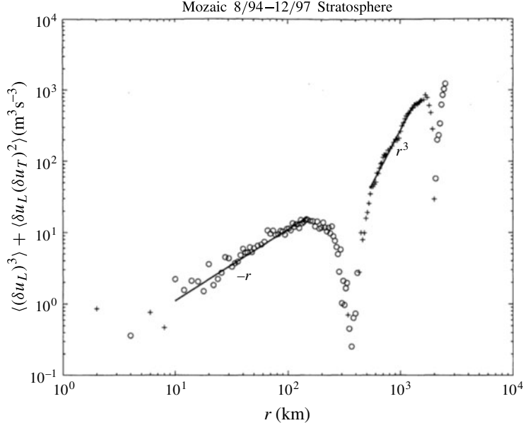
FIGURE 1. Sum of the diagonal third-order structure functions. Straight lines indicate the power laws -r and r^3 . Circles and crosses indicate negative and positive values, respectively. (Reproduced from Cho & Lindborg 2001.)
