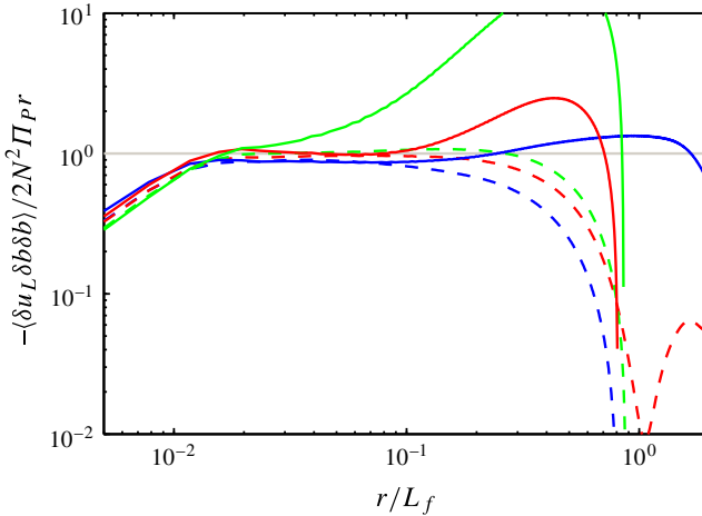
FIGURE 5. Plot of -\langle\delta u_L \delta b \delta b\rangle/2N^2 \Pi_p r for the different runs. Lines as in figure 4.
