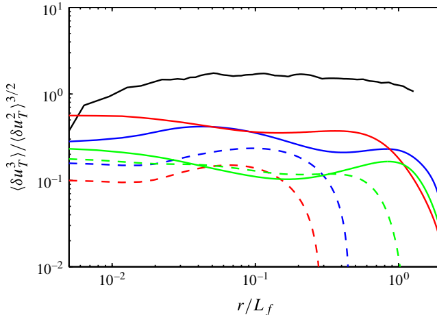
FIGURE 14. Plot of skewness \langle \delta u_T^3 \rangle / \langle \delta u_T^2 \rangle^{3/2} for the different simulations. Coloured lines as in figure 4; black line: measurements in the atmosphere (evaluated from Cho & Lindborg 2001). The separation distance for the atmospheric data has been normalized using L_f = 1000 km.
