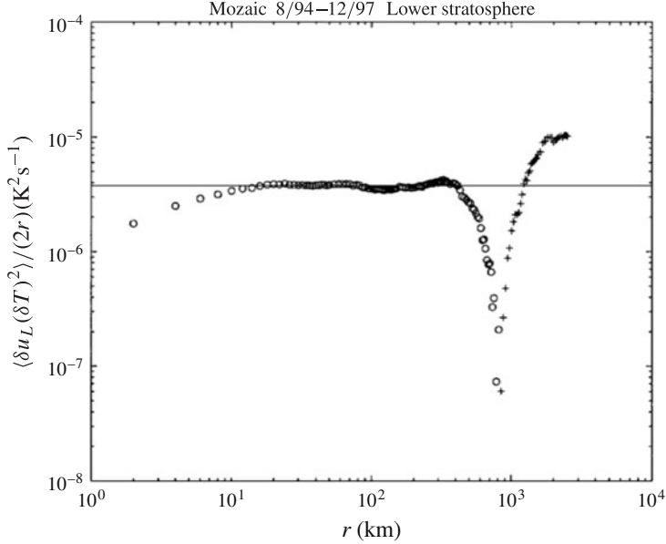
FIGURE 2. Plot of \langle \delta u_L \delta T \delta T \rangle / (2r) versus r . Solid line: best linear fit, 20 \text{ km} < r < 400 \text{ km} . Circles and crosses indicate negative and positive values, respectively. (Reproduced from Lindborg & Cho 2000.)
