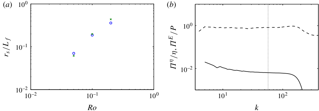
FIGURE 10. (Colour online) (a) Transition scale r_s at which \langle \delta u_L \delta \mathbf{u} \cdot \delta \mathbf{u} \rangle changes sign. \circ , Q-runs; \times , prediction of the transitional scale r_s = 2\pi\sqrt{\varepsilon/\eta} (Vallgren et al. 2011). (b) Flux of energy (—) and enstrophy (---) for the Q05 run. Vertical dotted line represents the transitional wavenumber k_s = 2\pi/r_s \approx 50 , i.e. k_s \approx 10k_f .
