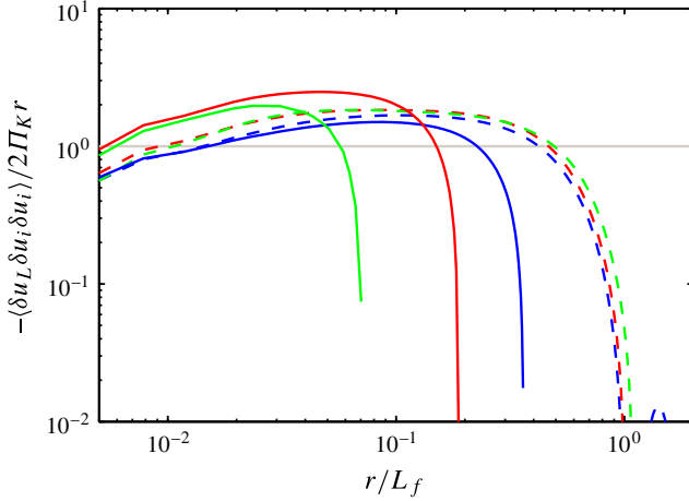
FIGURE 4. Plot of -\langle\delta u_L \delta u_i \delta u_i\rangle/2\Pi_K r for the different runs. Solid lines: Q -forcing; dashed lines: M -forcing. Green Ro = 0.05 ; red Ro = 0.1 ; blue Ro = 0.2 .
