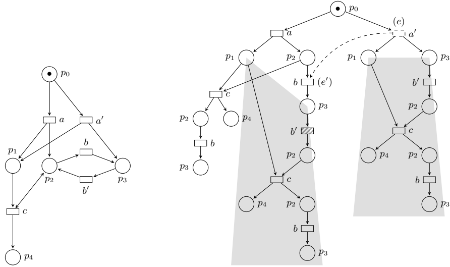
Fig. 2. A safe Petri net (left) and one of its branching processes (right). Configurations [e] and [e'] lead to the same marking \{p_1, p_3\} and have isomorphic extensions (in gray). The dashed arrow represents the fact that [e'] \triangleleft [e] . Consequently e is a cut-off.
