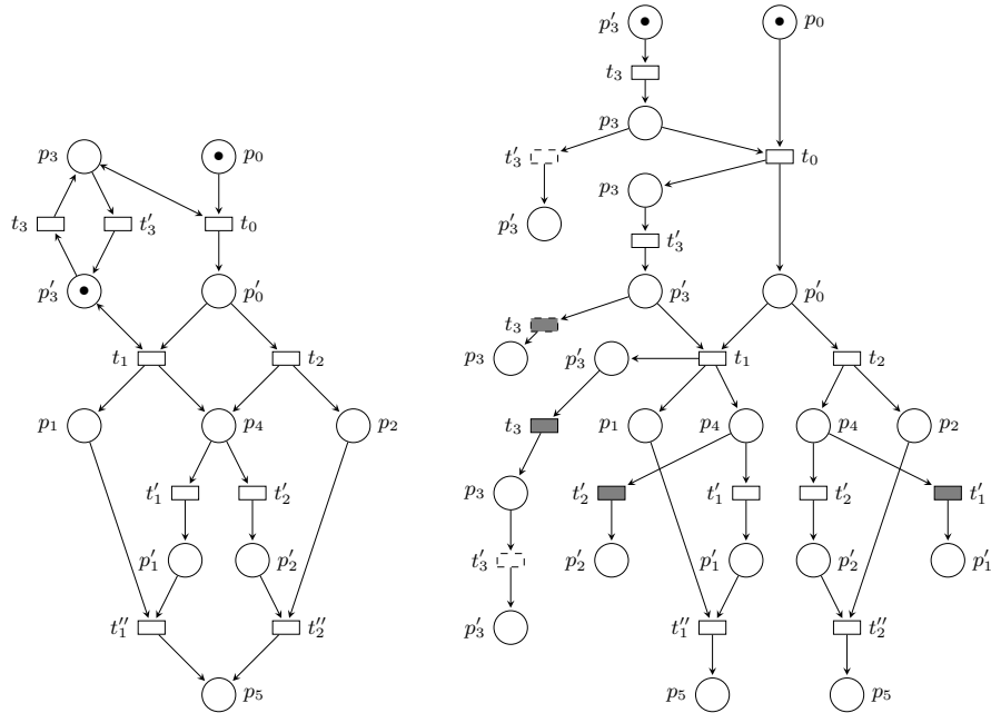
Fig. 1. A safe Petri net (left) and a finite complete prefix (right) of its unfolding. Dashed events are flagged as cut-offs : the unfolding procedure does not continue beyond them. Events in gray can be declared as useless by the reduction procedure for \{p'_3, p_5\} reachability, and can be skipped during the goal-driven prefix computation.
