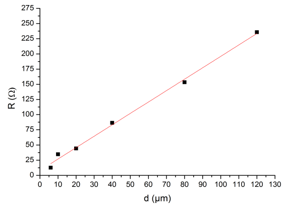
Figure 6. Evolution of resistance as a function of the distance between the contact pads for the same sample as in figure 5.
