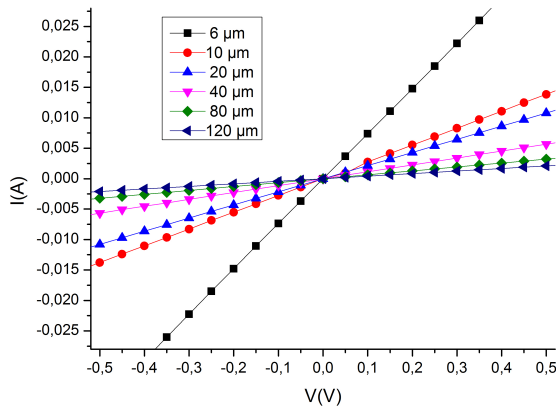
Figure 5. I-V characteristics of the sample for different distances between the contact pads of the TLM structure.
