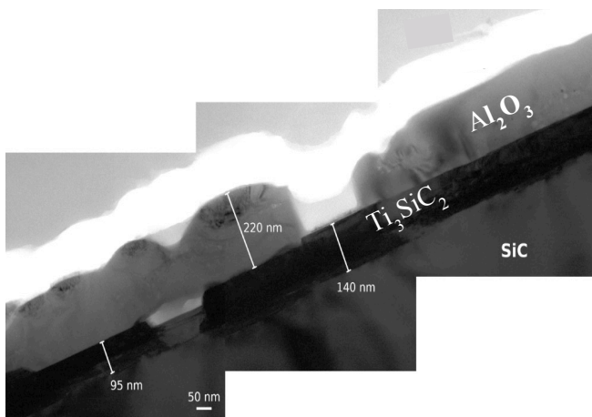
Figure 3. Cross-sectional TEM image of the same sample as in figure 1-a. \text{Ti}_3\text{SiC}_2 covers completely the surface of the SiC substrate and is itself covered by an Al oxide layer.
