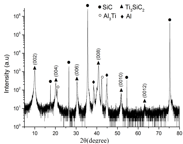
Figure 4. XRD pattern of the TiAl contacts onto 4H-SiC annealed at 1000°C for 10 min with proper baking of the system.
