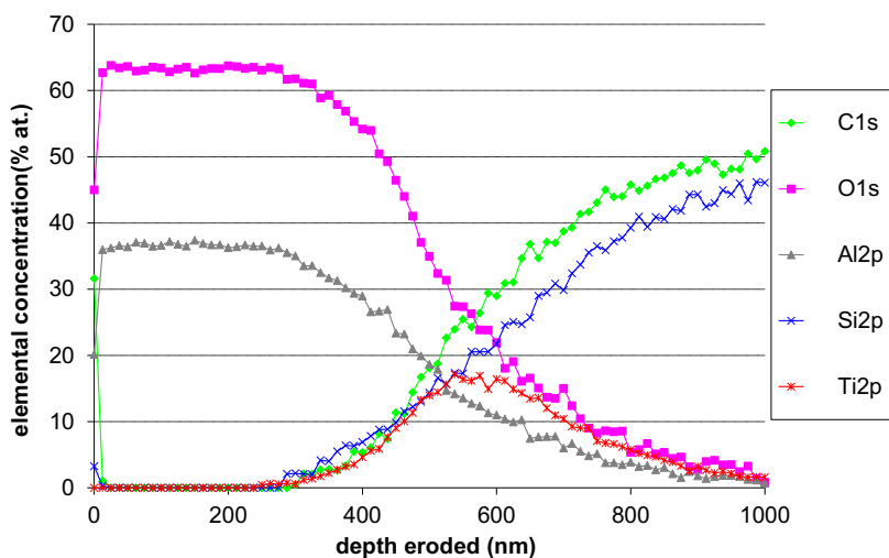
Figure 2. XPS depth profile of C, O, Al, Si and Ti of the TiAl contacts onto 4H-SiC annealed at 1000°C for 10 min.
