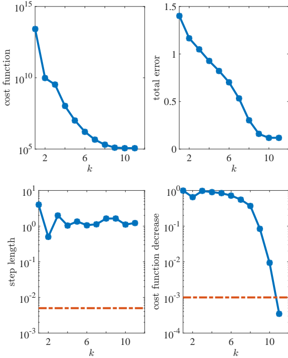
FIG. 6. Convergence of the algorithm for \alpha = 10^{-0.5} , c_{\text{gd}} = 1 \text{g}\cdot\text{cm}^{-3} , and N_0 = 10^7 photons. (Top left) cost function \mathcal{C} as a function of the iteration number k . (Top right) total normalized Euclidean error \text{error}_{\text{tot}} as a function of the iteration number k . (Bottom left) step length \lambda^{(k)} vs iteration number k . (Bottom right) cost function decrease \frac{\mathcal{C}^{(k-1)} - \mathcal{C}^{(k)}}{\mathcal{C}^{(k-1)}} vs iteration number. The red dashed lines indicate the values of the chosen stopping criteria.
