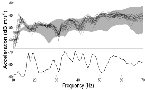
Fig. 24 Observation 2, zoom into band \mathcal{B}_L : experimental FRF measurements (black lines), random FRF using the identified ML-SROM (gray region), and OVL function (black line underneath)
