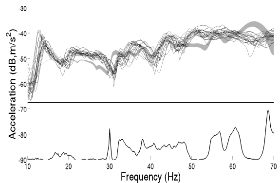
Fig. 14 Observation 2, zoom into band \mathcal{B}_C : experimental FRF measurements (black lines), random FRF using the identified C-SROM (gray region), and overlap function OVL (black line underneath)
