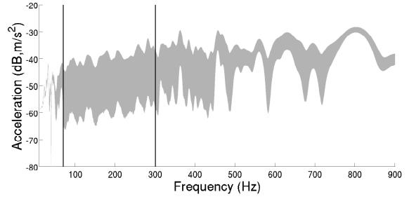
Fig. 26 Observation 1: random FRF using the identified ML-SROM but for which \delta^L = \delta^H = 0 is imposed.
