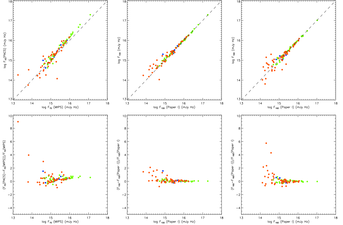
Fig. B.1. Left column: comparison of the MIPS and PACS 70\ \mu\text{m} fluxes. Middle and right columns: comparison of the PACS 100\ \mu\text{m} and 160\ \mu\text{m} fluxes presented in this paper and those published in Paper I.
