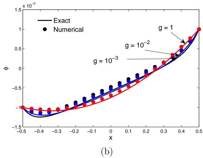
Figure 6. Solution field along the layer thickness for a fixed flexoelectric coefficient f = 0.01 and a varying strain gradient coefficient g ; (a) Displacement; (b) electric potential.
