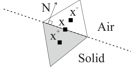
Figure 2. Two adjacent elements across the interface between the solid and surrounding media for the approximation of the Maxwell stress jump across the interface.
