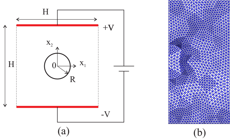
Figure 8. Soft cylindrical body subjected to an electric field; (a) geometry; (b) FEM mesh.
