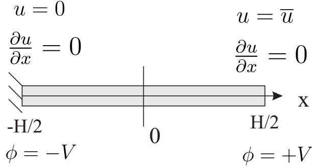
Figure 5. Layer with flexoelectric properties subjected to voltage.
