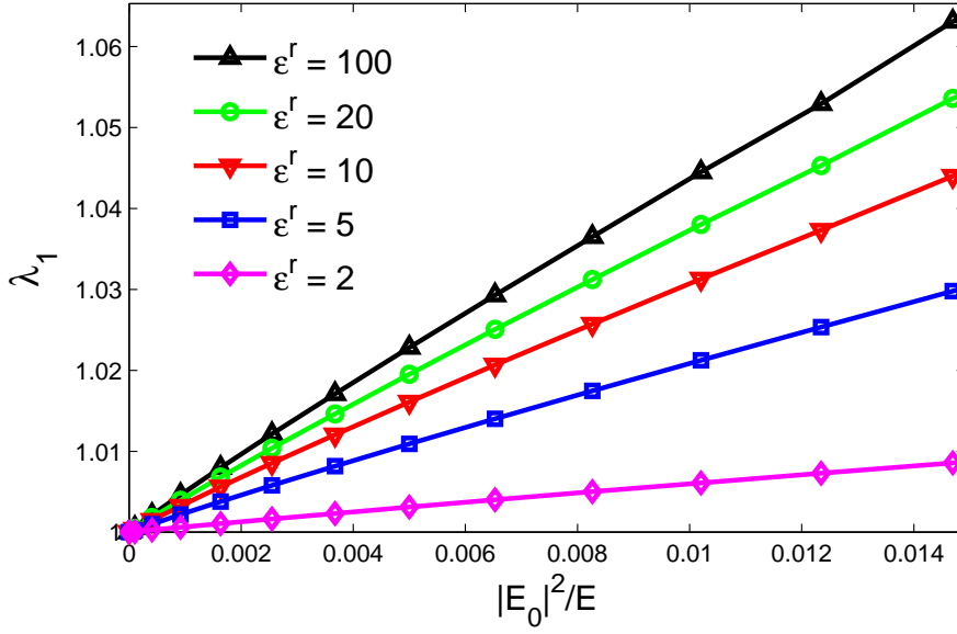
Figure 10. Stretch of the initial spherical particle as a function of the applied electric current |\mathbf{E}_0|^2 .
