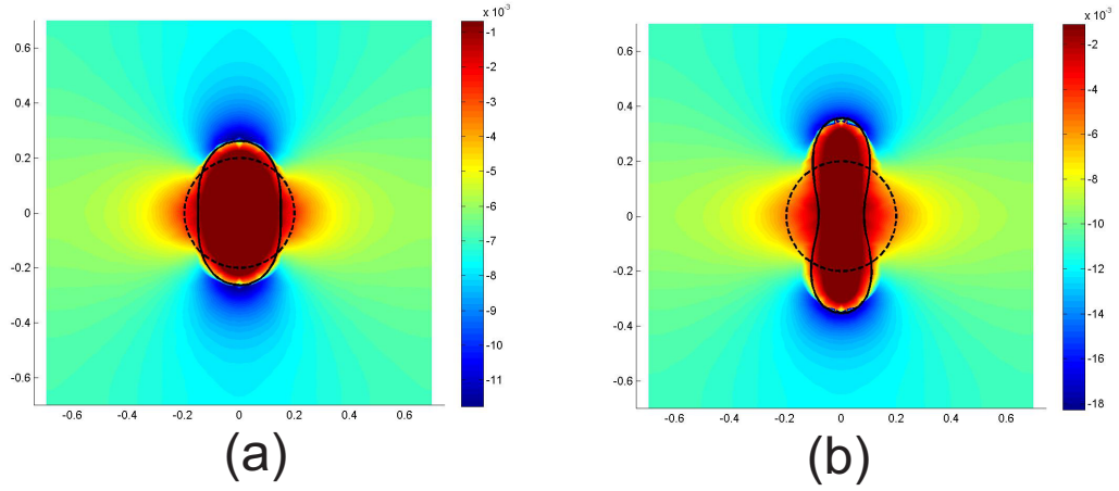
Figure 9. Electric field \tilde{E}(\mathbf{x})_2 and deformed configuration of the ellipsoid (magnified 10 times) for an applied electric field (a) E_0 = 0.009 V/m and (b) E_0 = 0.141 V/m, \epsilon_r = 20 , E = 0.01 MPa, \nu = 0.45 .
