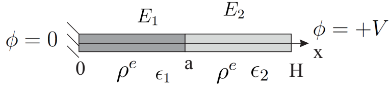
Figure 3. Bilayer material with uniform charge \rho subjected to voltage.
