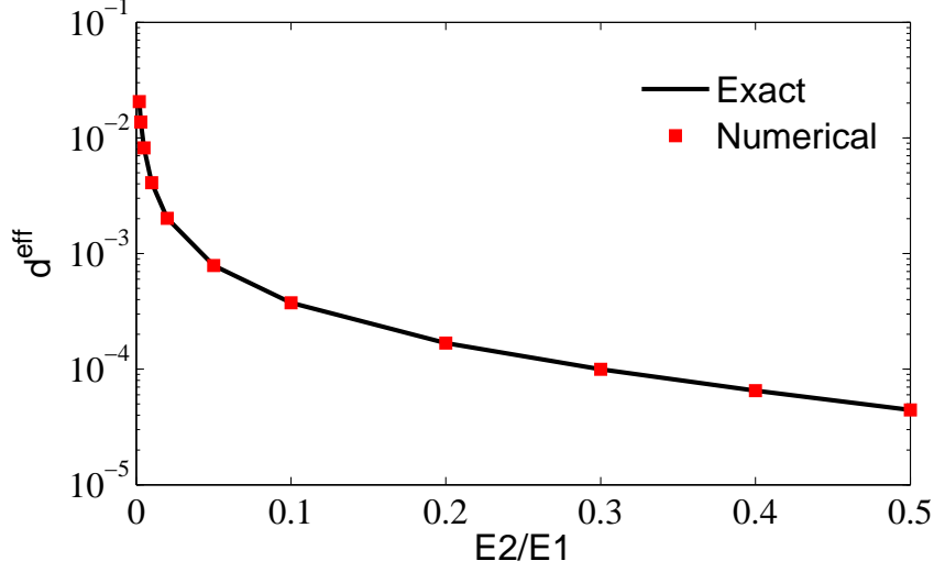
Figure 4. Effective piezoelectric coefficient d^{\text{eff}} as a function of the ratio E_2/E_1 .
