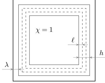
FIGURE 2. Localizing on thin shells for the square LQ .
