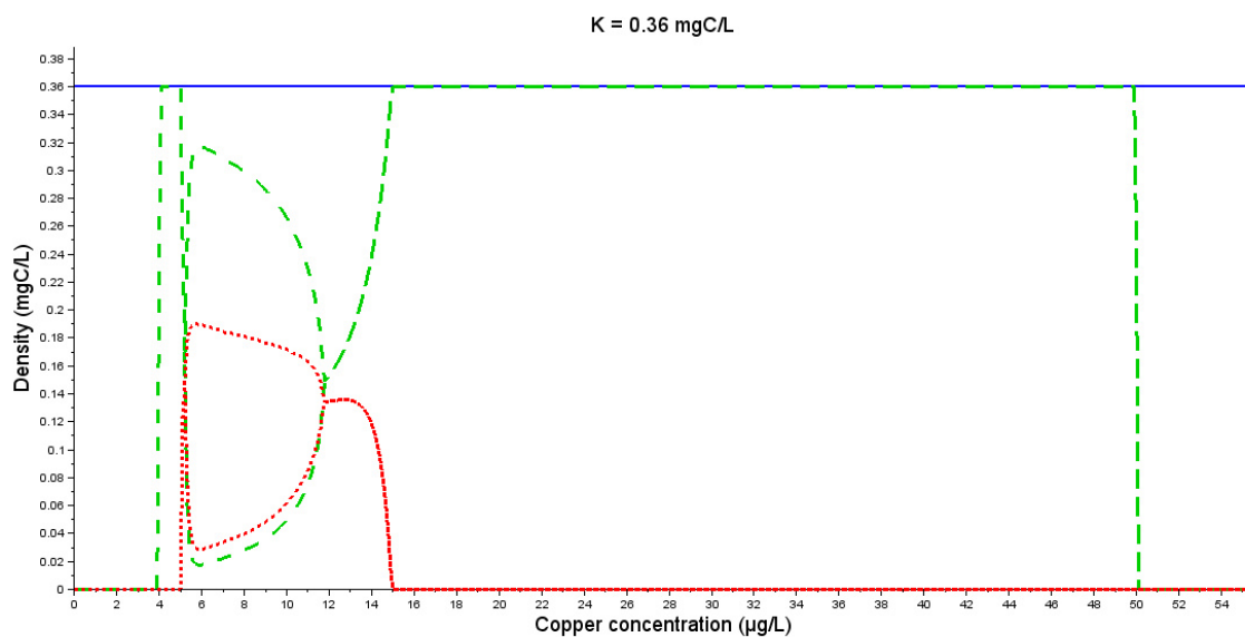
Figure 3. Scenedesmus (dashes) and Daphnia (dotted lines) equilibrium values for copper concentrations ranging between 0 and 55 \mu\text{g Cu/L} . Solid line: carrying capacity. The two lines per population between 5.2 and 11.8 \mu\text{g Cu/L} show the oscillations' minima and maxima.
