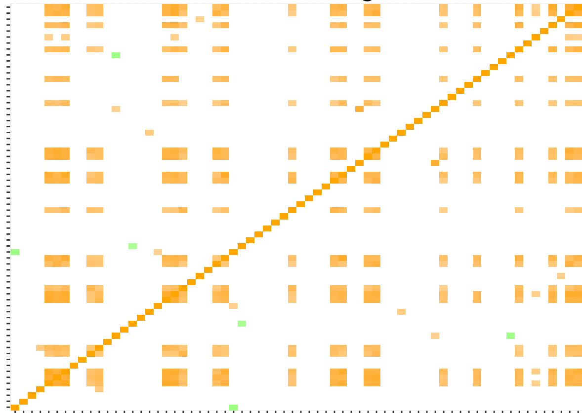
thresholding
