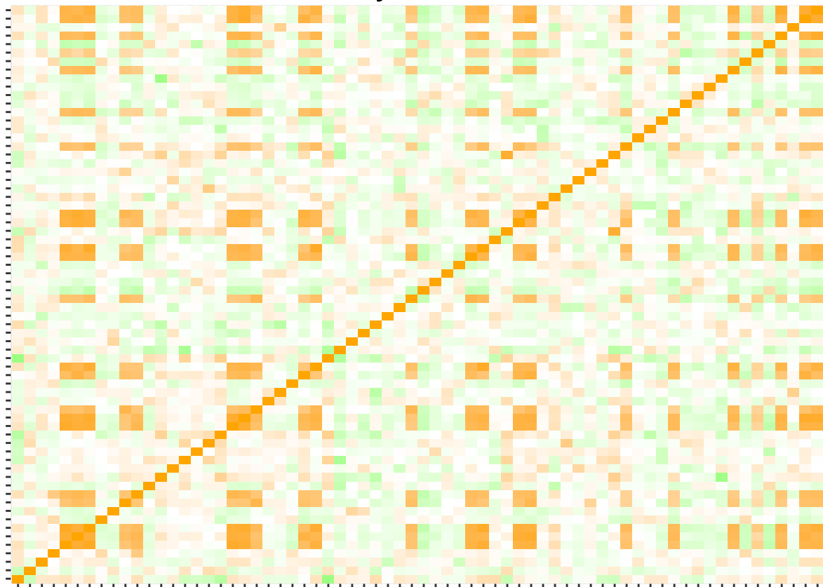
similarity calculation
