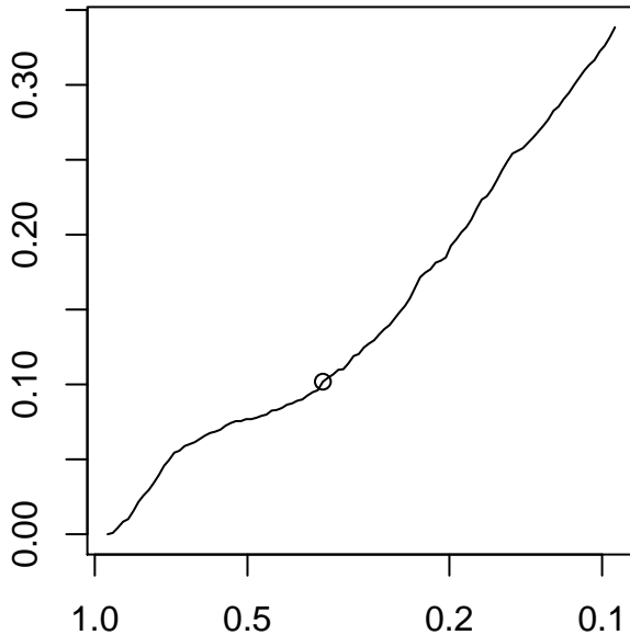
Solution path sparsity levels
