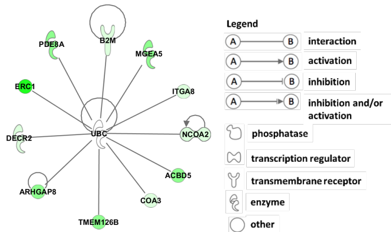
Fig. 13 IPA network including all the 11 annotated genes of cluster 2.
