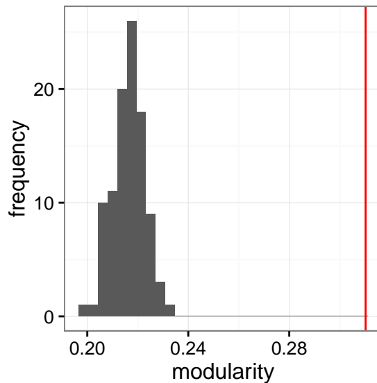
Fig. 12 Distribution of the maximum modularity over 100 random graphs with the same degree distribution as the “55-eqtl network” compared to the maximum modularity found for this network (red vertical line).
