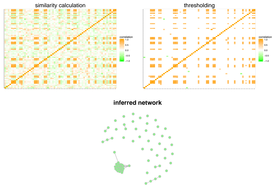
Fig. 3 Main steps in network inference.
