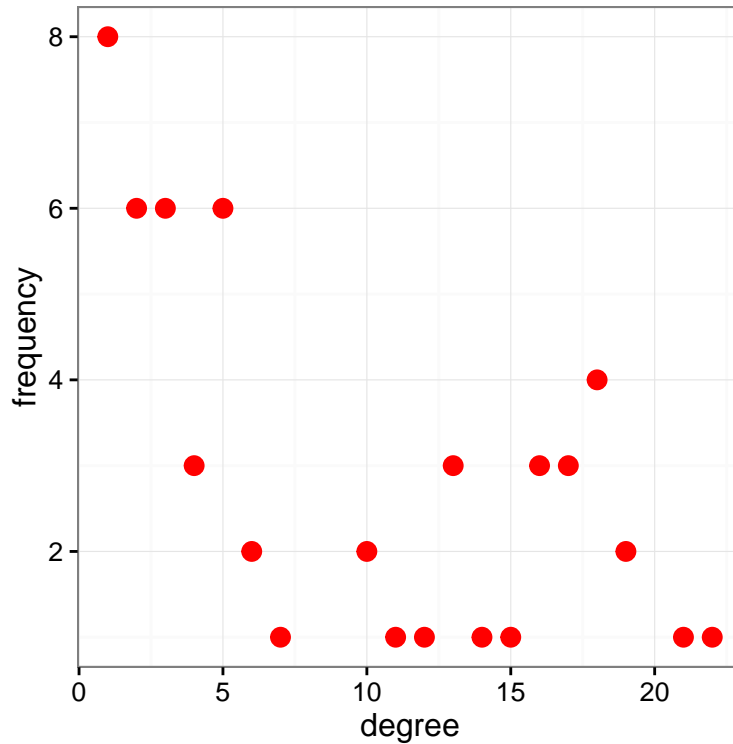
Fig. 8 Degree distribution for the “55-eqtl network”.
