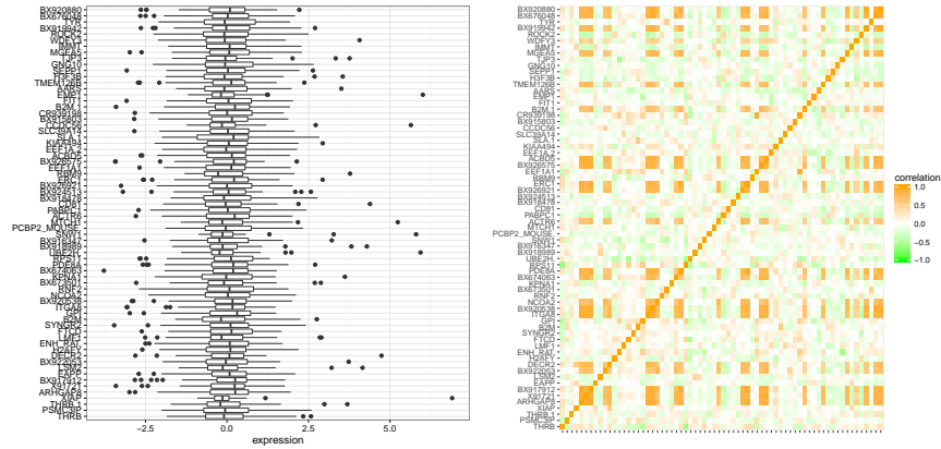
Fig. 2 Left: boxplot of the gene expression distributions (68 genes). Right: heatmap of the correlation matrix between pairs of genes expression.
