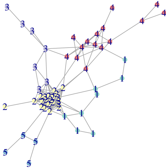
Fig. 11 Partition of the “55-eqtl network” into 5 modules. The colours and labels indicate module membership.
