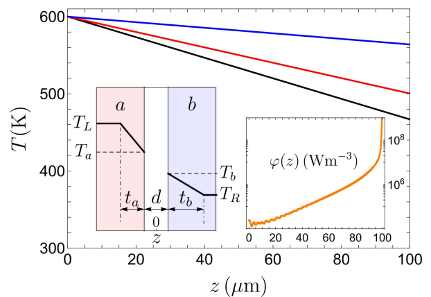
FIG. 1. The left inset shows a schematic of two parallel slabs separated by a distance d along the z direction ( z = 0 denotes the middle of the gap). The two slabs exhibit a temperature profile T(z) : the temperature is constant and has values T_L and T_R in the regions z \leq -d/2 - t_a and z \geq d/2 + t_b , respectively, and variable in the regions -d/2 - t_a < z < -d/2 and d/2 < z < d/2 + t_b , with T_a and T_b denoting the temperatures at the slab–vacuum interfaces. In the main part of the figure, temperature profile along the temperature-varying region of the hot slab in a configuration involving two silica slabs with t_a = t_b = 100 \mu\text{m} held at external temperatures T_L = 600 \text{ K} and T_R = 300 \text{ K} at the outer ends, and separated by vacuum gaps d . The points z = 0, 100 \mu\text{m} represent the boundary of the thermostat and the interface with the vacuum gap. The three lines correspond to d = 10 \text{ nm} (black), 20 \text{ nm} (red) and 50 \text{ nm} (blue). The right inset shows the z -dependent radiative flux-rate \varphi(z_a) (see text) along slab a at d = 100 \text{ nm} .
