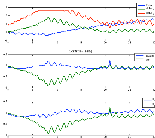
Fig. 10. Angles and controls with respect the time (in sec.) during the trajectory described in Fig. 9. The middle plot shows the components H_{\parallel} and H_{\perp} of the control, whereas the bottom plot shows the H_x and H_y components, in the reference basis.
