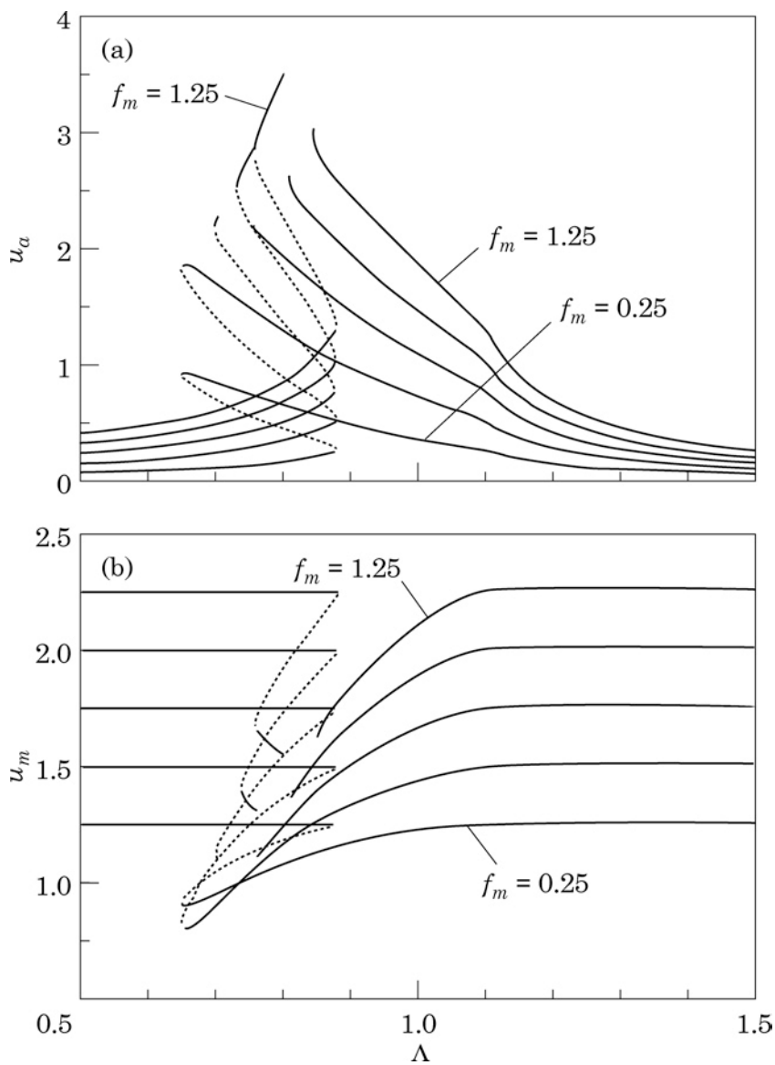
Figure 14. The effect of the preload f_m on the (a) alternating u_a and (b) mean u_m components of the steady state forced response for f_m \in [0.25, 1.25] with an increment of 0.25, \zeta = 0.05 and w_a = 0.25 . —, Stable solutions; \cdots , unstable solutions.
