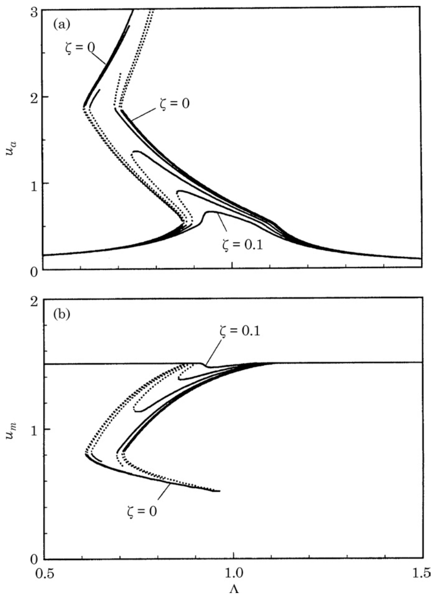
Figure 13. The effect of the damping ratio \zeta on the (a) alternating u_a and (b) mean u_m components of the steady state forced response for \zeta \in [0, 0.1] with an increment of 0.02, f_m = 0.5 and w_a = 0.25 . —, Stable solutions; \cdots , unstable solutions.
