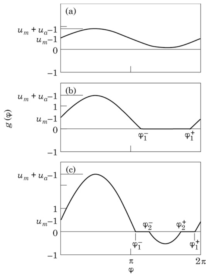
Figure 2. Non-linear restoring function g(\varphi) for (a) no-impact ( NI ), (b) single sided impact ( SSI ) and (c) double sided impact regimes ( DSI ).
