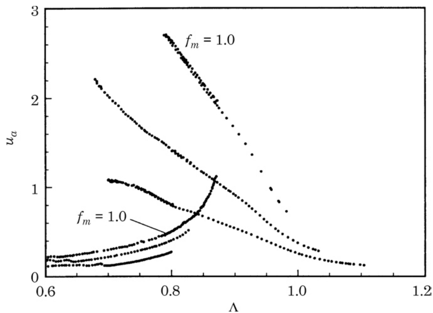
Figure 15. The effect of the preload f_m on the measured alternating component u_a of the steady state forced response for f_m \simeq 1.0 , 0.5 and 0.25 , w_a \simeq 0.20 and \zeta \simeq 0.01 .
