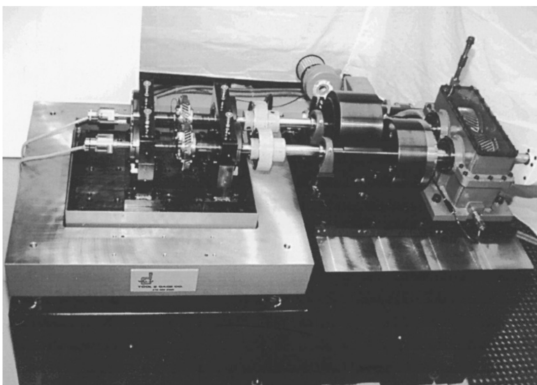
Figure 4. The experimental test rig.
