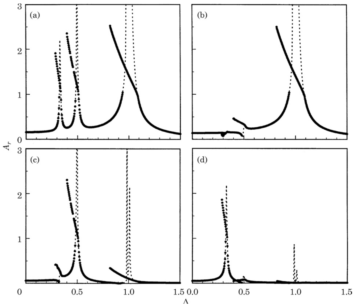
Figure 10. A comparison of the harmonic content of multiple term HBM solutions (●) with the corresponding LTV system results (---); (a) A_{rms} versus A ; (b) A_1 versus A ; (c) A_2 versus A ; (d) A_3 versus A . The system parameters are the same as in Figure 7.
