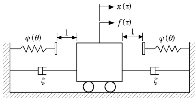
Figure 1. The physical system: a mechanical oscillator of unit mass.
