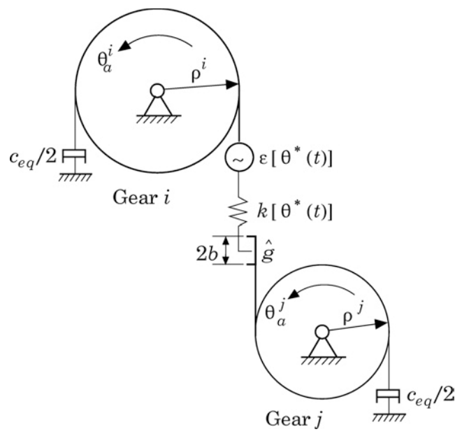
Figure 3. An application example: a single-DOF torsional model of a gear pair.
