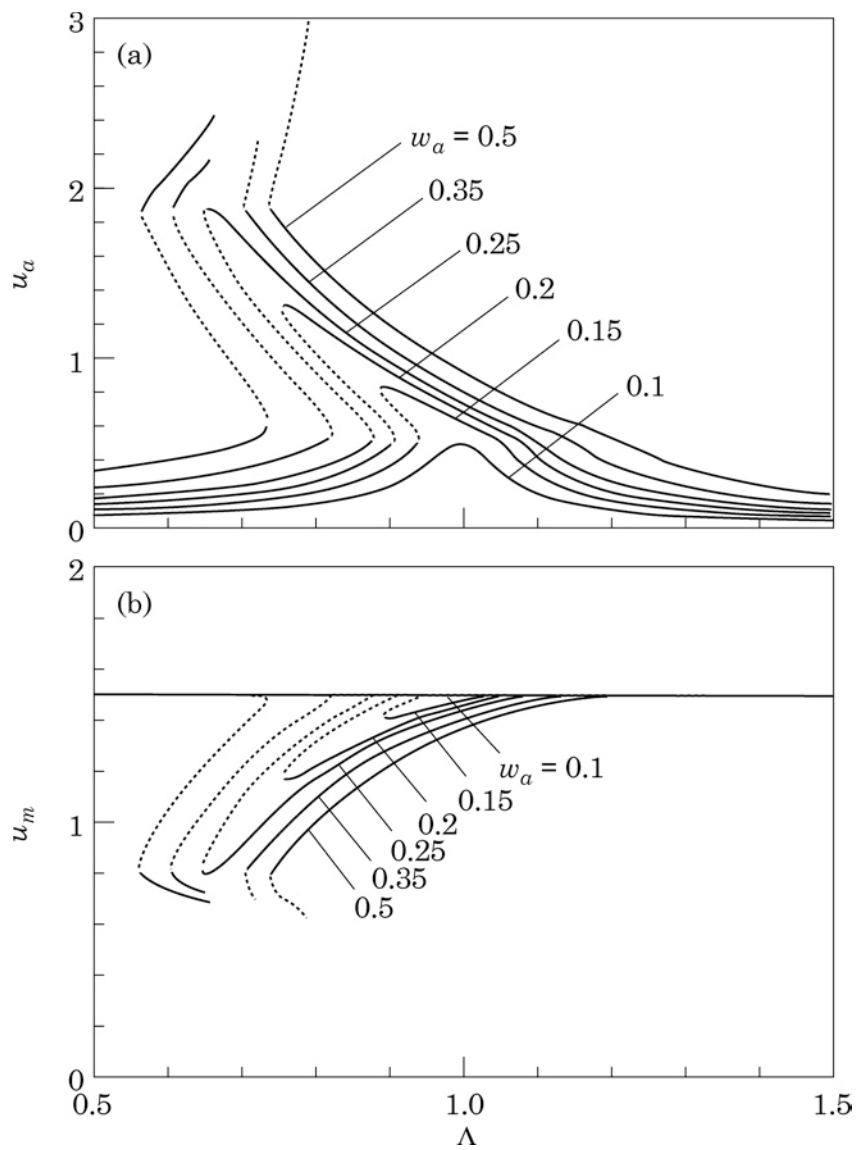
Figure 11. The effect of stiffness variation w_a on the (a) alternating u_a and (b) mean u_m components of the steady state forced response for w_a \in [0.1, 0.5] , f_m = 0.5 , and \zeta = 0.05 . —, Stable solutions; \cdots , unstable solutions.
