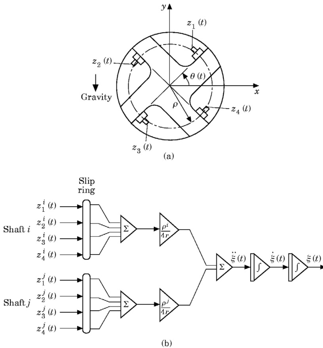
Figure 6. (a) The arrangement of linear accelerometers on a gear wheel and (b) the block diagram of the analog circuitry used to compute \zeta(t) from measured accelerometer signals z_i(t) .
