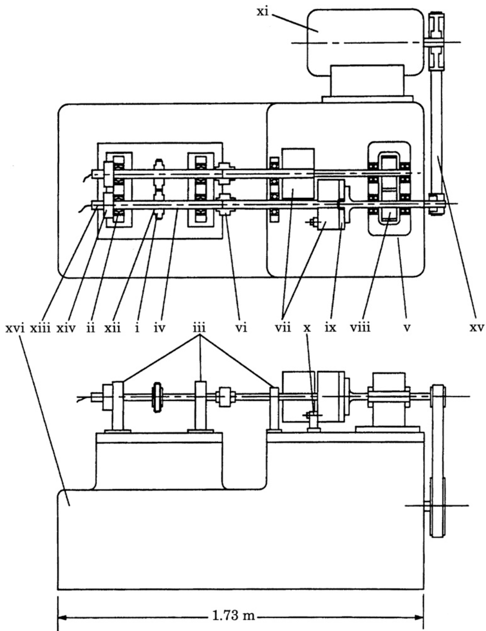
Figure 5. A schematic of the test rig: i, test gear pair (AGMA Class 14); ii, ultra-precision spherical roller bearings; iii, rigid bearing pedestals to reduce structural dynamics; iv, test gear shafts that are very stiff in bending and torsion; v, slave gear box necessary for power recirculation; vi, compliant elastomer couplings and vii, flywheels for torsional isolation between test and slave gears; viii, slave gears with topological modifications for reduced excitation; ix, split hub; x, locking pin for torque adjustment; xi, 20 hp DC motor with electronic speed control; xii, location of torsional accelerometers; xiii, slip rings to connect accelerometer signals to conditioning amplifiers; xiv, optical encoders (18 000 lines) to control data sampling rates; xv, drive belt; xvi, polymer granite base.
