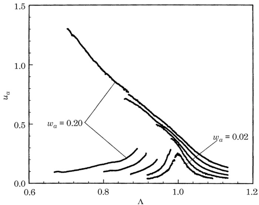
Figure 12. The effect of stiffness variation w_a on the measured alternating component u_a of the steady state forced response for w_a \simeq 0.20, 0.15, 0.10, 0.05 and 0.02 , \zeta \simeq 0.01 and f_m = 0.5 .
