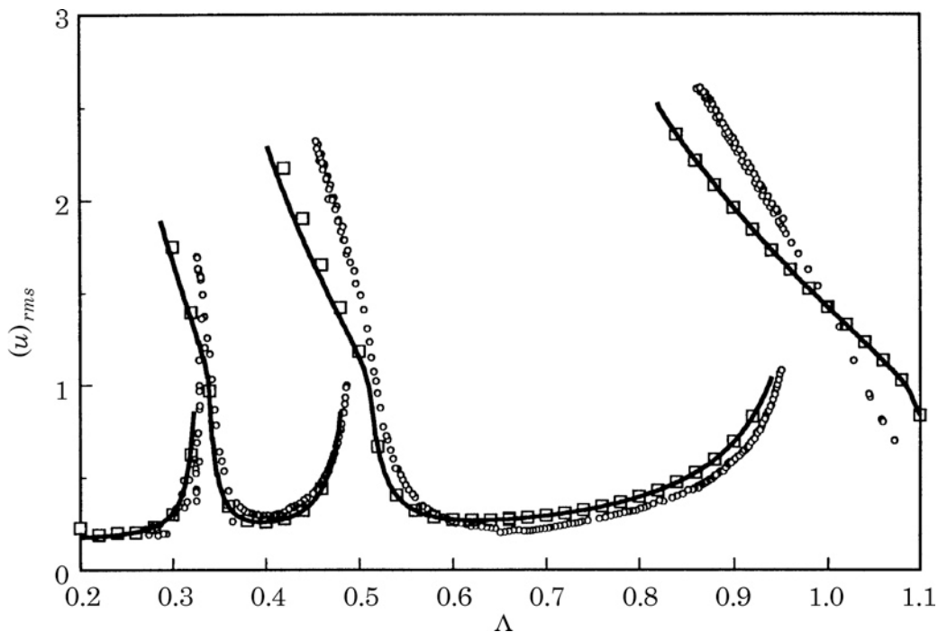
Figure 7. A comparison of HBM solutions (—) with numerical integration ( \square ) and experimental ( \circ ) results. R=3 , K=3 , with w_2=0.15 , w_4=0.075 , w_6=0.06 and all other w_i=0 , f_1=1.0 with all other f_i=0 , and \zeta=0.01 .
