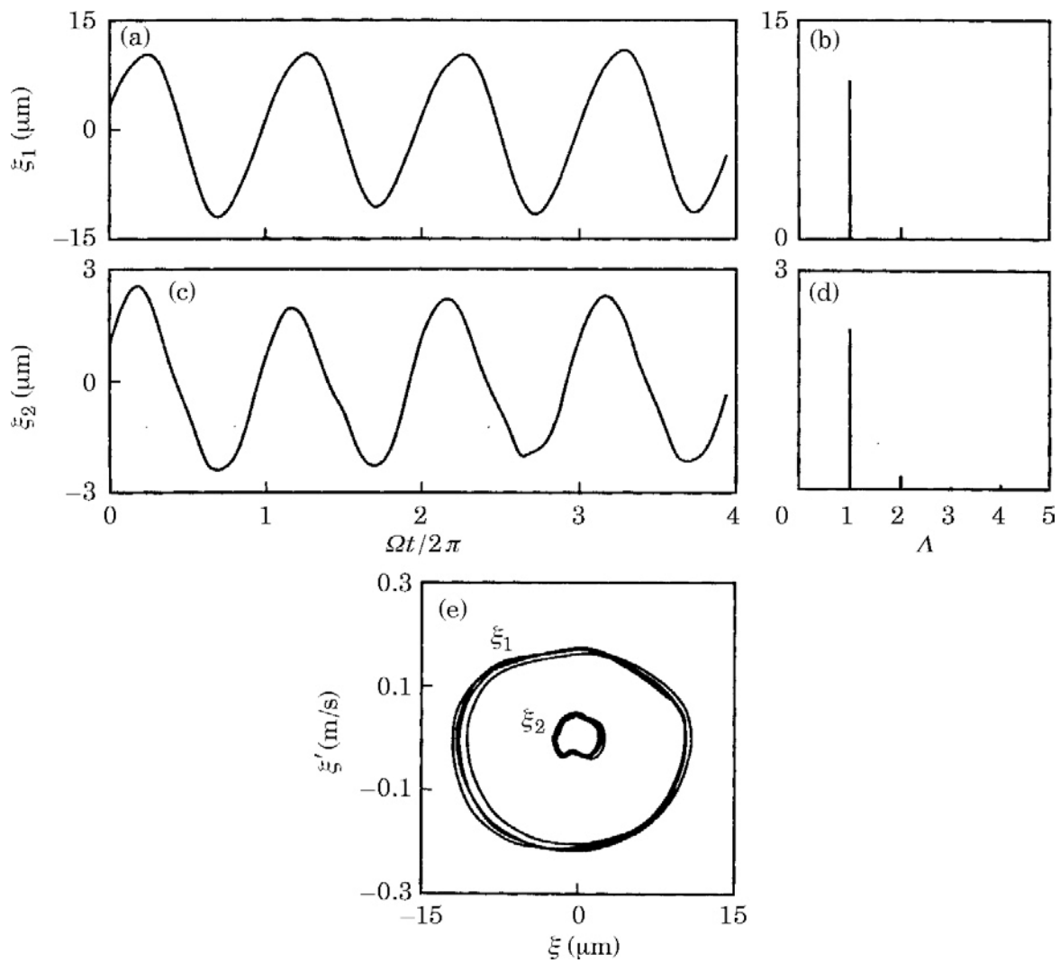
Figure 8. Measured coexisting steady state solutions \xi_1(t) and \xi_2(t) at \Lambda=0.9 : (a) \xi_1(t) versus \Omega t/2\pi ; (b) FFT of \xi_1(t) ; (c) \xi_2(t) versus \Omega t/2\pi ; (d) the FFT of \xi_2(t) ; and (e) phase portraits \xi_1'(t) versus \xi_1(t) and \xi_2'(t) versus \xi_2(t) . The system parameters are the same as in Figure 7.
