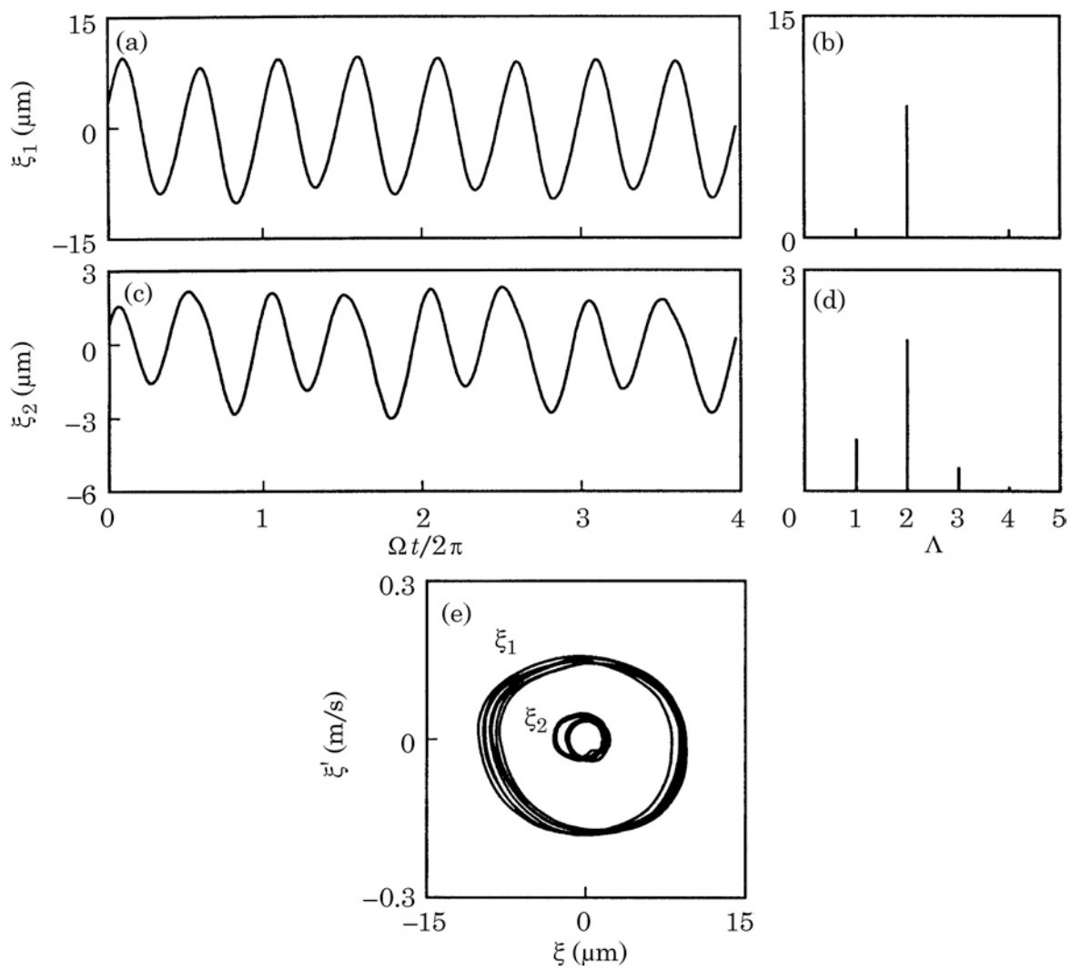
Figure 9. Measured coexisting steady state solutions \xi_1(t) and \xi_2(t) at \Lambda=0.45 : (a) \xi_1(t) versus \Omega t/2\pi ; (b) the FFT of \xi_1(t) ; (c) \xi_2(t) versus \Omega t/2\pi ; (d) the FFT of \xi_2(t) ; (e) phase portraits \xi_1'(t) versus \xi_1(t) and \xi_2'(t) versus \xi_2(t) . The system parameters are the same as in Figure 7.
