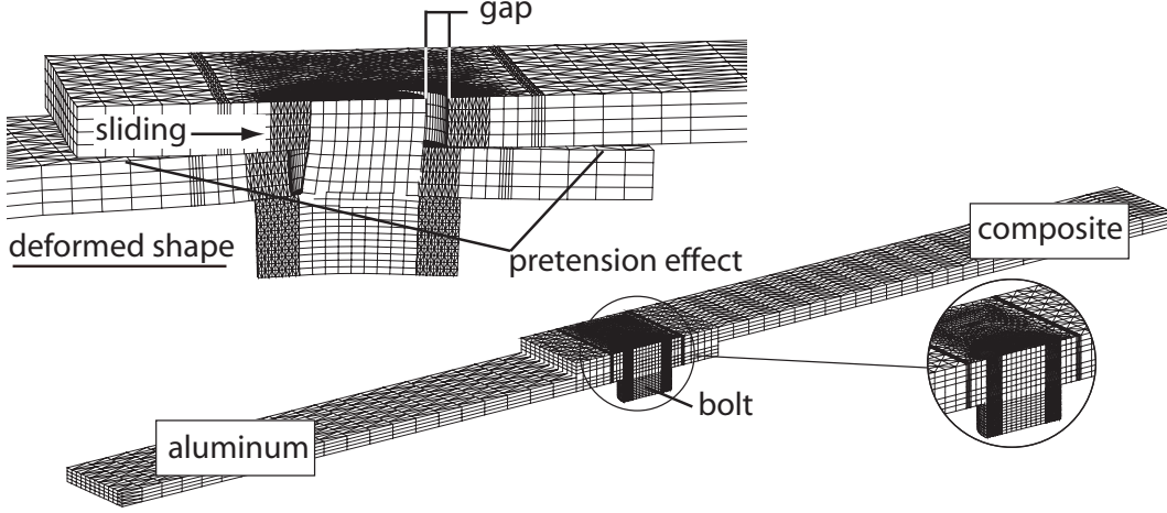
Figure 1: Bolted joint - mesomodel
