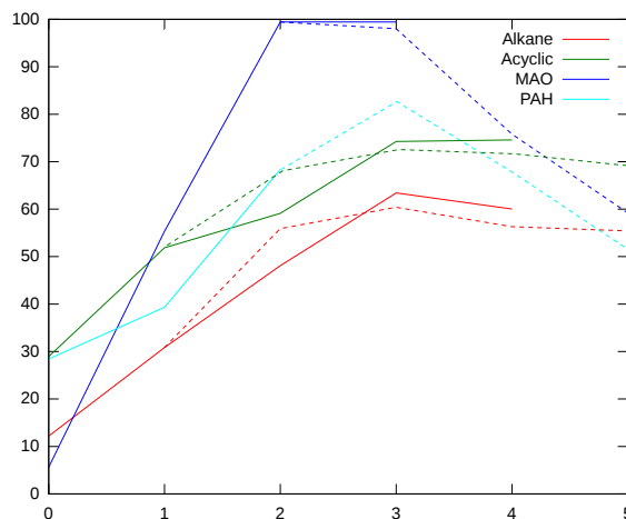
Fig. 2. Gain in accuracy compared to Riesen [8] obtained for each dataset versus the size of considered paths ( k ). Smashed lines represents the gain using beam search algorithm instead of A^* algorithm.
