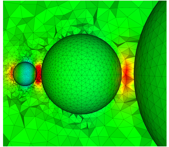
(c) \mathbb{P}_3
