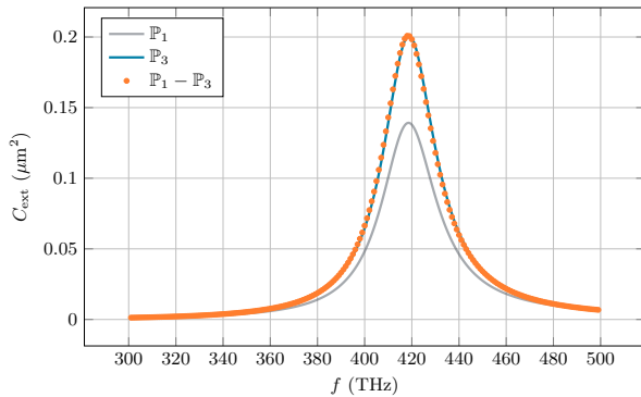
Figure 14: Extinction cross-section of the bowtie nanoantenna obtained with \mathbb{P}_1 , \mathbb{P}_3 and \mathbb{P}_1 - \mathbb{P}_3 approximations. Less than 2 % of relative error is observed between full \mathbb{P}_3 and \mathbb{P}_1 - \mathbb{P}_3 computations, for a speedup factor superior to 2.
