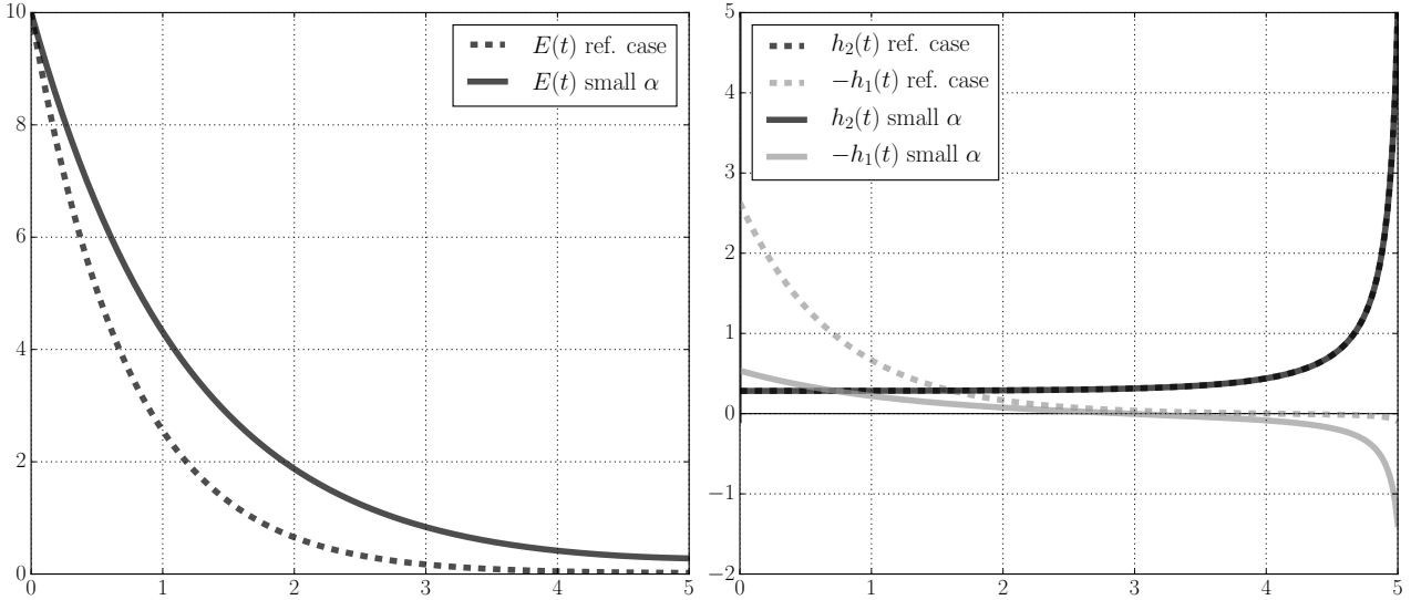
Figure 2: Comparison of the dynamics of E (left) and -h_1 and h_2 (right) between the “reference” parameters of Figure 1 and smaller \alpha (i.e. \alpha = 0.1 instead of 0.4 ) such that |h_1(0)| is smaller.
