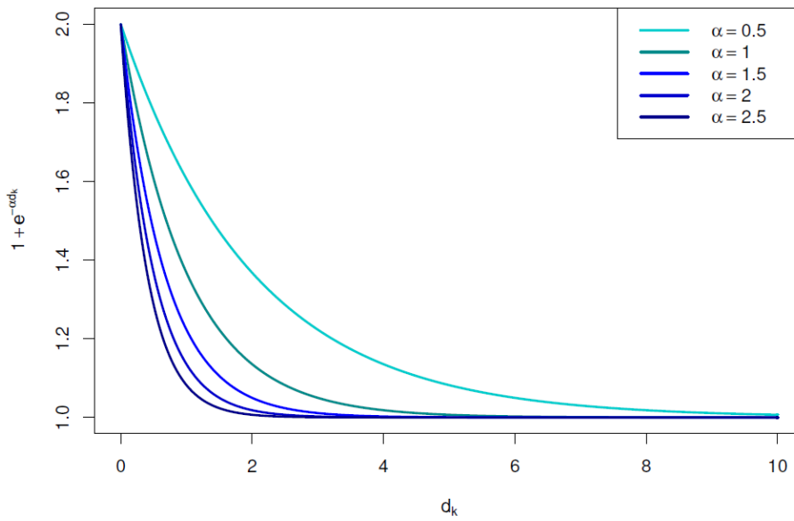
FIGURE 2.5. Evolution of the penalization coefficient (1 + e^{-\alpha d_k}) according to d_k , for different values of \alpha .
