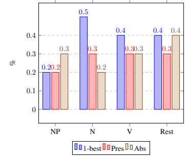
(c) Average translation posterior entropy per unit group (WMT'14 SMT)
