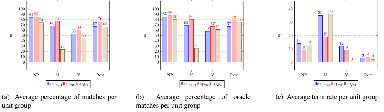
Figure 2: Translation quality statistics for Cochrane SMT
