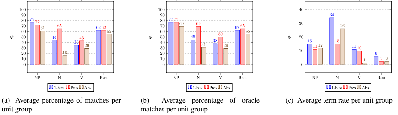
Figure 3: Translation quality statistics for WMT'14 SMT
