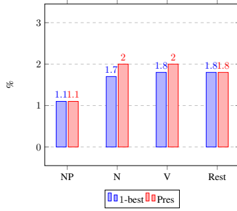
(a) Average translation prior entropy per unit group (Cochrane SMT)
