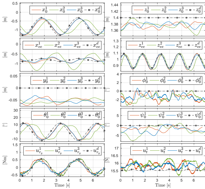
Fig. 6: Experimental results for trajectory (b) (see Fig. 4.b). Same color and line code is used as in Fig. 5. The proposed controller (blue) achieves always a better tracking performance. An interesting result is that for such a dynamic tracking task, the controller with the static compensation (green) performs worse than the one with minimum compensation (red).
