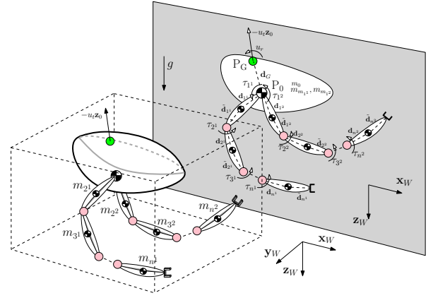
Fig. 1: Sketch of a protocentric aerial manipulator (PAM) with two arms, described with the same notation of [12]. Notice that in the 3D model of the PAM (the one on the left down), the axis of rotation for each individual joint of each arm is parallel to \mathbf{y}_W . Hence its projection on \mathbf{x}_W - \mathbf{z}_W plane looks like the one in the grayed area (right up). Notice the possibility that the geometric center of base actuation, P_G , and the CoM of the flying base, P_0 are not coinciding in the same point.
