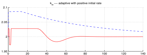
Figure 8: Adaptive gain K_\omega . Dashed: without mgt proportional gain adaptation; Solid: with mgt proportional gain adaptation.
