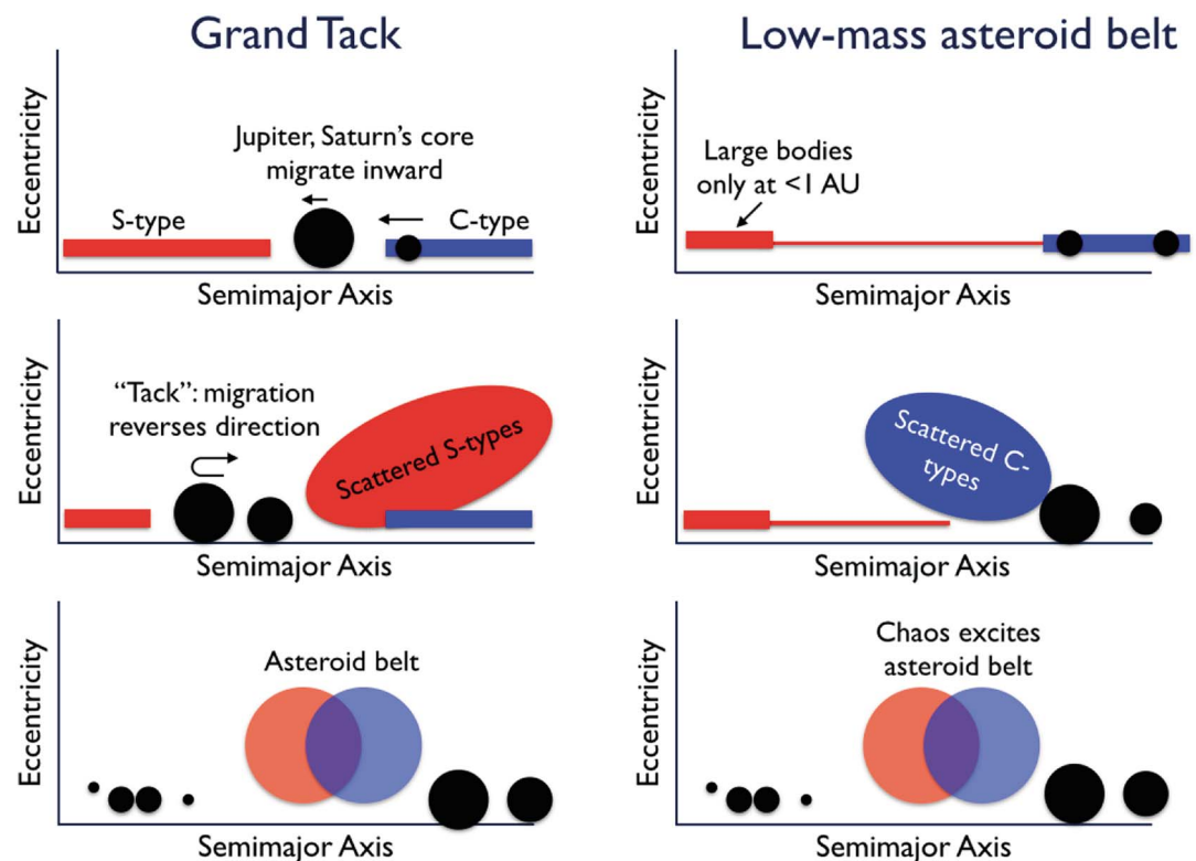
Figure 4. Cartoon representation comparing (left) the Grand Tack model with (right) a model in which the asteroid belt was low mass even at early times. While the evolution of the two models is quite different, each can match the present-day inner solar system.
