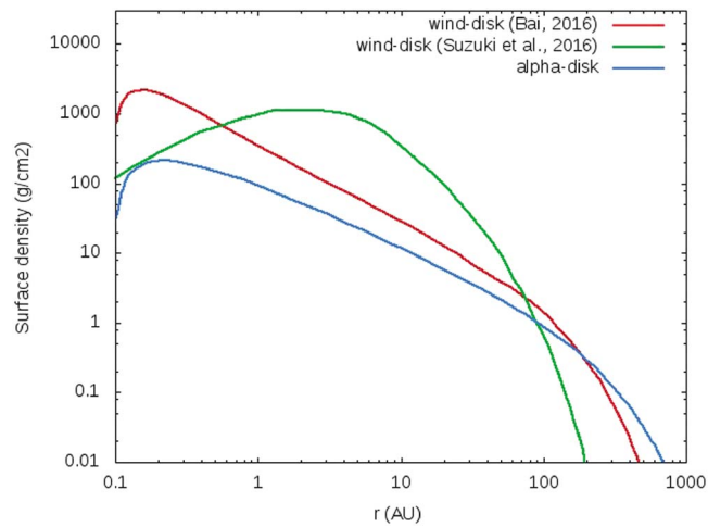
Figure 1. Structure of different disk models, all with an accretion rate on the star of \sim 5 \times 10^{-9} M_{\odot}/\text{y} . Each curve shows the surface density as a function of heliocentric distance. Two models of low-viscosity disks where transport is dominated by winds are shown, from Bai [2016] (red color; \alpha = 2 \times 10^{-4} ) and Suzuki et al. [2016] (green color; \alpha = 8 \times 10^{-5} ). They are labeled as “wind disks” to contrast with the classic \alpha disk, whose density distribution is also shown in blue. In the \alpha disk model the surface density of the gas scales inversely to the assumed viscosity (here \alpha = 0.01 is assumed). Note the depletion of gas in the inner part of the disk in the Suzuki et al. model.
