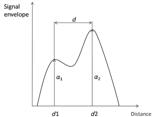
Fig. 2 Two-point sources.
