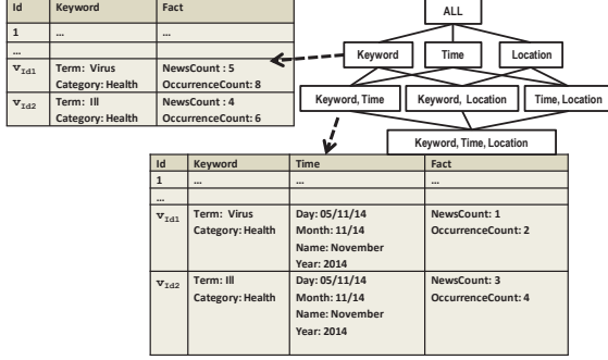
Figure 7: Implementing the pre-computed aggregation lattice into a column-oriented NoSQL logical model.
