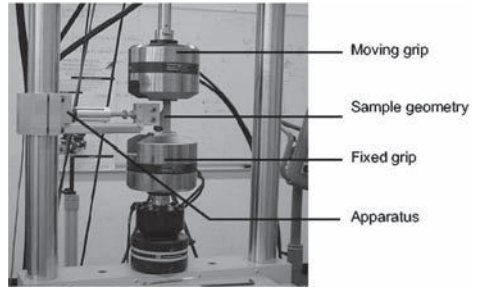
Figure 5. Experimental set-up.
