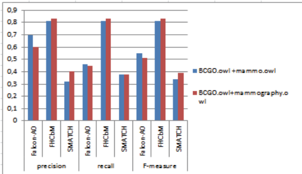
Figure 8: Synthesis of FHCbM, Falcon and SMatch methods- Precision, Recall and F-measure
