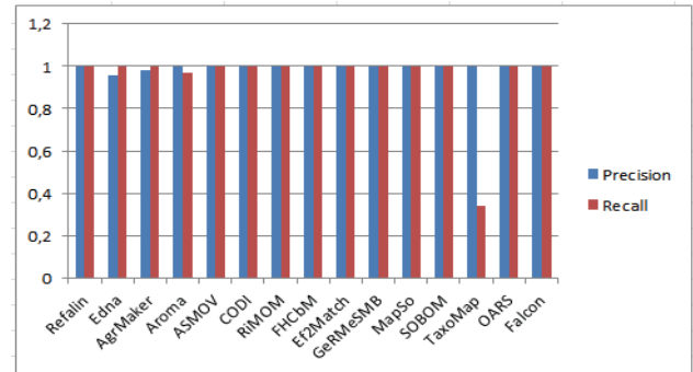
Figure 3: Evaluation results on group 1xx.
