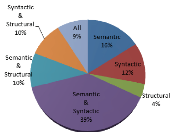
Figure 10: Percentages of the alignments found by the different similarity techniques (among correct alignments)
