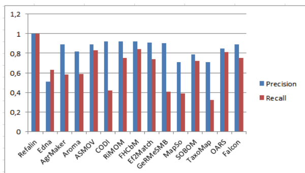
Figure 5: Evaluation results on group 3xx.
