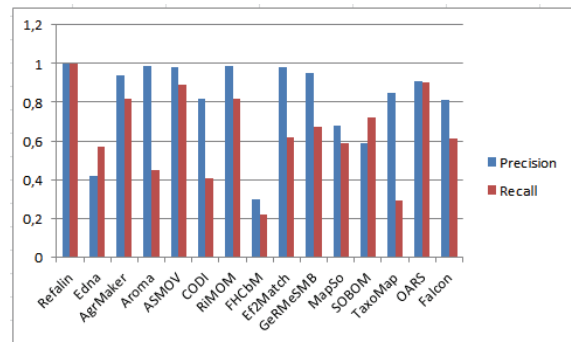
Figure 4: Evaluation results on group 2xx.
