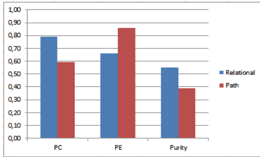
Figure 6: Performance evaluation of the fuzzy clustering based on both ontologies distances
