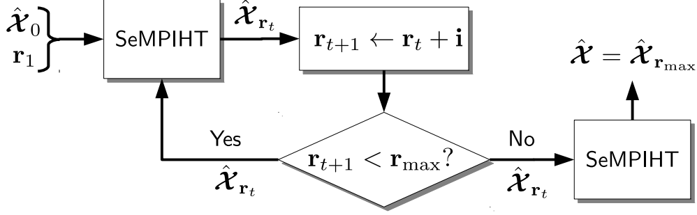
Figure 1: Diagram of SeMPIHT algorithm with GRI heuristic.
