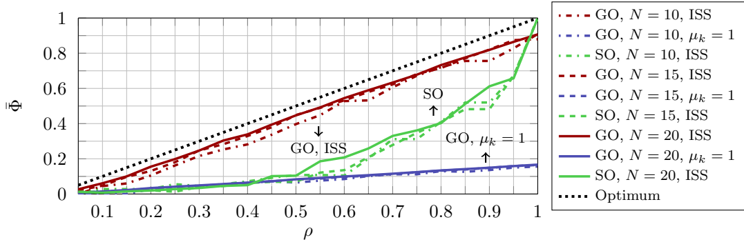
Figure 4: Estimated (normalized) number of DOF which can be recovered by SeMPIHT for each level of \rho , using Gaussian MOs (GO) and sampling MOs (SO). Recovery was successful in all 15 realizations for values of \bar{\Phi} below or over the curve.
