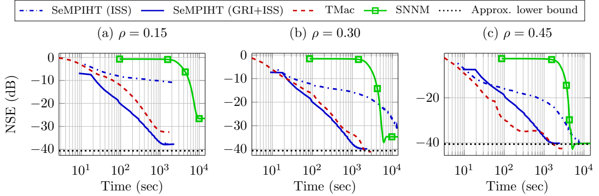
Figure 9: Performance of TC algorithms in the reconstruction of the 1024 \times 1344 \times 33 hyperspectral image Gualtar scene [15], which is uniformly sampled at random with subsampling rate \rho .
