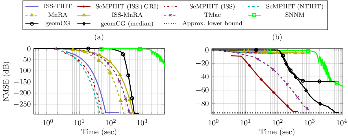
Figure 7: Convergence of several algorithms in a TC scenario where \rho = 0.2 and N_1 = N_2 = N_3 = 300 : (a) T1 tensors of mrank \mathbf{r} = (30, 30, 30) ; (b) T2 tensors ( \varphi = 2 ) modeled with mrank \mathbf{r} = (90, 90, 90) .
