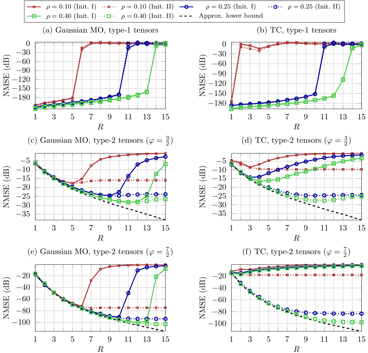
Figure 3: Effect of GRI on recovery performance of SeMPIHT with Gaussian ((a), (c) and (e)) sensing and in TC ((b), (d) and (f)). The approximate lower bound in (c)–(f) is computed as \text{NMSE}(\mathcal{S}_{\mathbf{r}}(\mathcal{X}^*); \mathcal{X}^*) .
