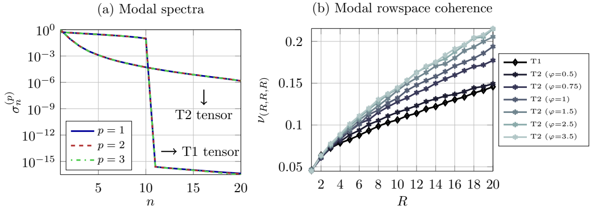
Figure 2: Typical behavior of the considered random tensor models: (a) modal singular spectra; (b) row space coherence (see (35)).
