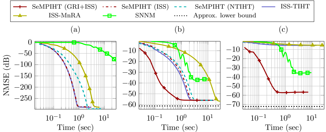
Figure 6: Convergence of several algorithms in a Gaussian sensing scenario where \rho = 0.25 and N_1 = N_2 = N_3 = 20 : (a) T1 tensors of mrank \mathbf{r} = (3, 3, 3) ; (b) T2 tensors ( \varphi = 2.5 ) modeled with mrank \mathbf{r} = (9, 9, 9) ; (c) T2 tensors ( \varphi = 2.5 ) modeled with mrank \mathbf{r} = (13, 13, 13) .
