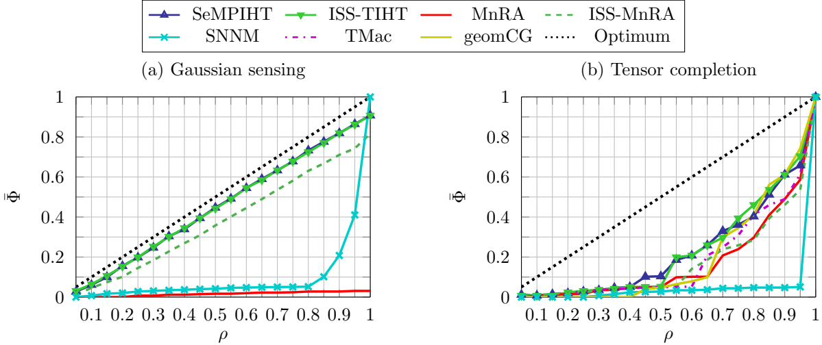
Figure 5: Estimated (normalized) number of DOF which can be recovered by several algorithms for each level of \rho , using Gaussian MOs (a) and sampling MOs (b). The measured tensors have dimensions N_p = 20 for all p . Recovery was successful in all 15 realizations for values of \bar{\Phi} below or over the curve.
