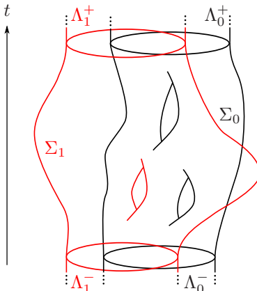
FIGURE 1. Two Lagrangian cobordisms inside a symplectisation \mathbb{R} \times Y , where the vertical axis corresponds to the \mathbb{R} -coordinate.
