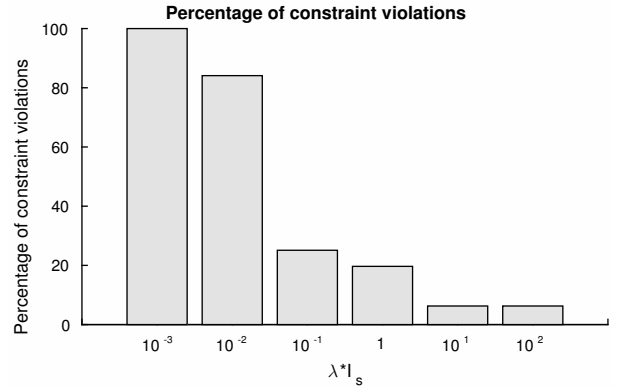
Fig. 4. Fraction of time at which the devices violate the interference constraints. The higher is \lambda , the higher is the penalty in case of interference constraint violations. This results in less violations by the mobile devices.
