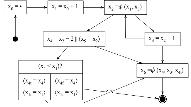
Figure 6. Figure 3 transformed by the rules in Figure 5.
