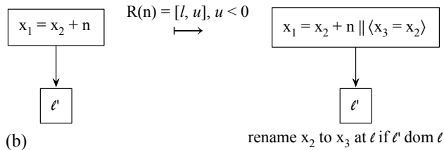
Figure 5. Transformation rules used to convert the syntax in Figure 2 into the syntax in Figure 4.
