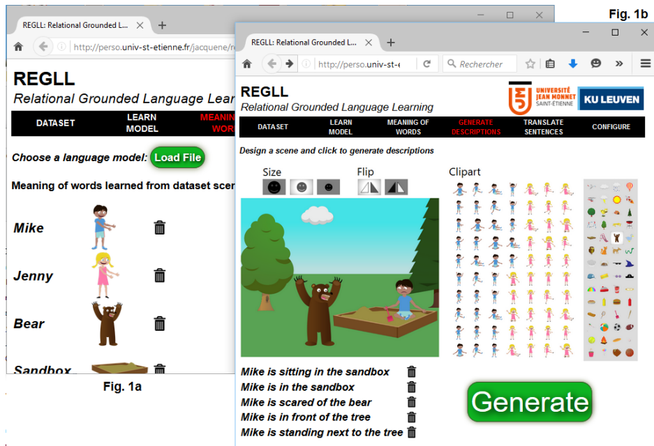
Fig. 1. Screenshots of the ReGLL interface.
