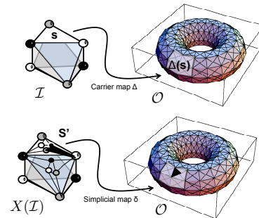
Fig. 7. The wait-free computability theorem, Fig 11.7 from [18].
