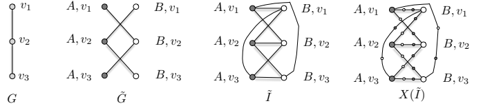
Fig. 6. G and colored graph \tilde{G} , with input \tilde{I} and views after one round X(\tilde{I}) , for robots A, B
