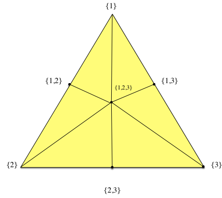
Fig. 9. Colorless executions of at least three processes starting on 1, 2, 3.
