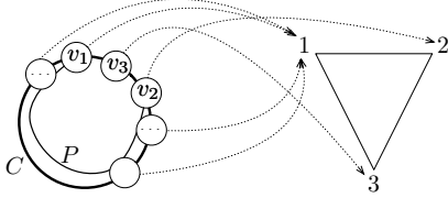
Fig. 3. Mapping vertices of the cycle C to values for Set Agreement
