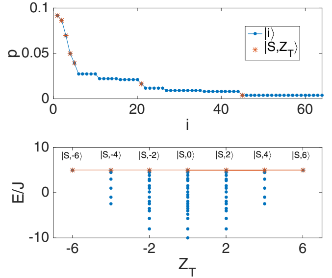
FIG. 6. (Top) The probabilities of all the H_{XXZ} eigenstates, as computed from \rho_{\text{NESS}} for L = 6 and J = U . (Bottom) The corresponding eigenenergies as a function of their magnetization. Highlighted are the |S, Z_T\rangle states. The system parameters are g = 0.1J , \kappa = 0.5g , and P = J .
