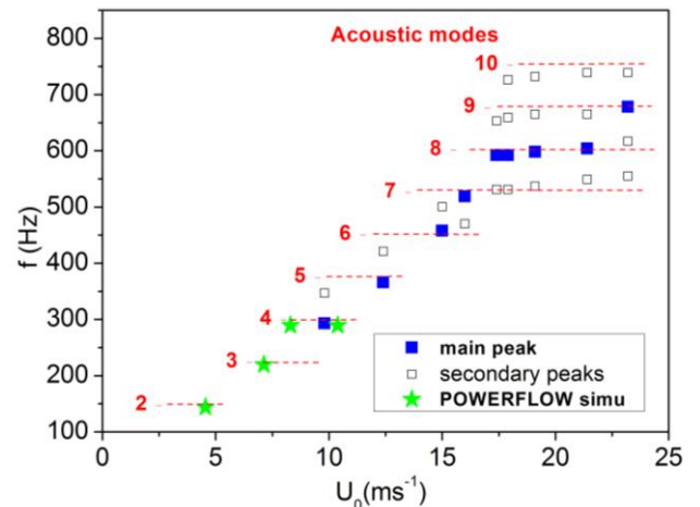
Figure 9 – Acoustic modes in the corrugated pipe. Experiments (in blue) and PowerFlow simulations (corrugated channel + chambers).
