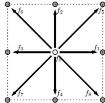
Figure 2 – Discrete probability density function with respect to the nine possible velocities for the particles in the D2Q9 case.
