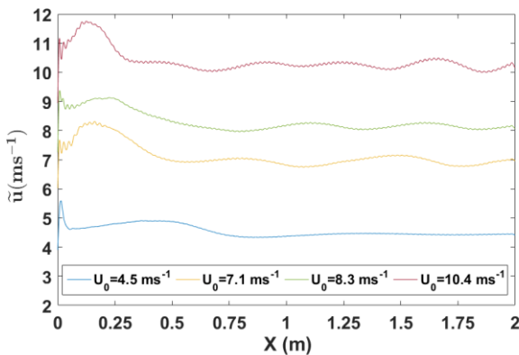
Figure 7 – Simulation results for corrugated channel + chambers. Time averaged mean velocity \tilde{u} with respect to the position X along to the symmetry axis of the corrugated pipe for the set of calculations.
