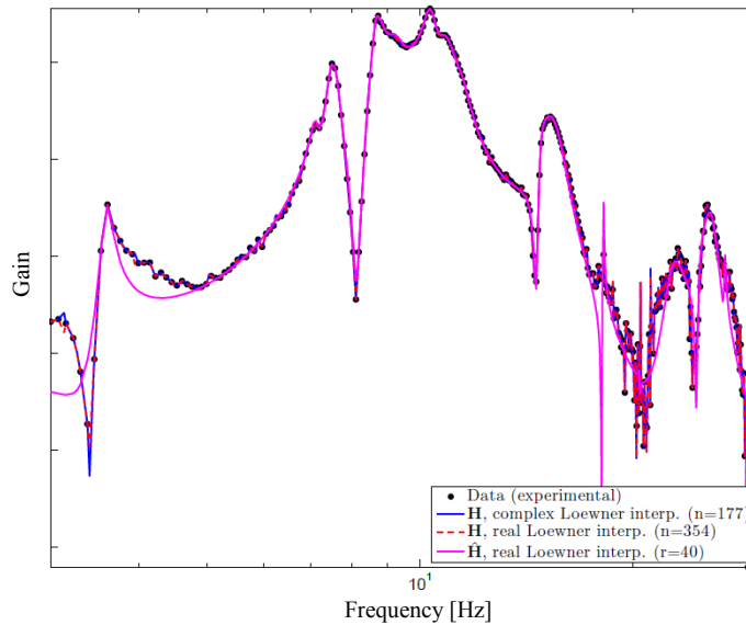
Figure 10: Illustration of the interpolatory results obtained by the Loewner approach on an open-loop frequency set obtained in experiments (SISO case)
