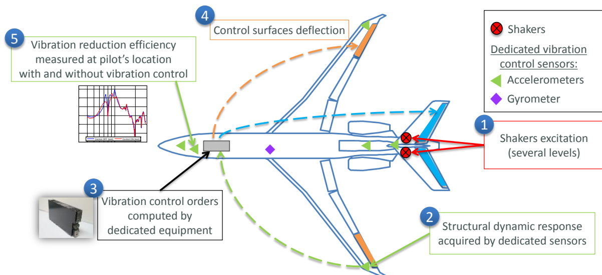
Figure 7 : Ground vibration test sequence
