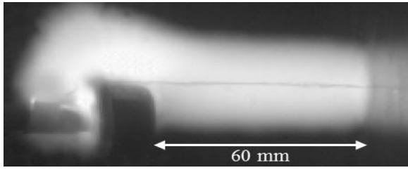
Fig. 3 Example of arc picture taken at 15 \mu s after the current triggering. The jet diverter electrode is located on the left-hand side and the aluminum panel is on the right-hand side (resolution: 0.46 mm/pixel; exposure time: 0.3 \mu s)
