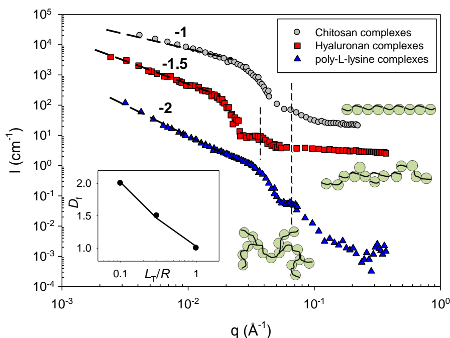
Fig. 4a. (Color on-line) SANS profiles collected at high ionic strength, I , and 20°C of the three PEL complexes: 0.01g/l chitosan/10g/l SiNP, 0.01g/l HA/2g/l SiNP, and 0.01g/l PLL/10g/l SiNP (monophasic and representative of domain III in D 2 O) solutions are prepared in the presence of 0.2M CH 3 COONa, 0.1M NaCl, and 0.2M KBr, respectively. For clarity, hyaluronan and chitosan complexes spectra have been shifted by two and three log units along the y-axis with respect to that of PLL complexes, respectively. All curves exhibit the first oscillation associated to the form factor of the SiNPs cross-section occurring around 6.5 \times 10^{-2}
