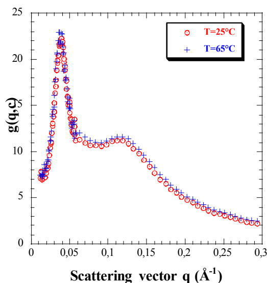
Figure 4. Scattering functions of the same NaPSS star solution (S100-S91 in D 2 O at c = 0.480 \text{ mol} \cdot \text{L}^{-1} – \phi = 5.34\% ; c > c^* = 0.075 \text{ mol} \cdot \text{L}^{-1} – \phi^* = 0.83\% ) at two distinct temperatures 25 °C (circles) and 65 °C (crosses).
